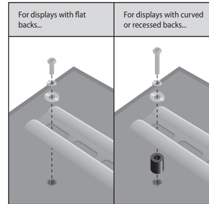
Fig. 4 - Use a longer bolt and spacer for displays with curved or recessed backs. Do not use the M6 Washer (O) if you are using the M8 Bolts (J or K).
