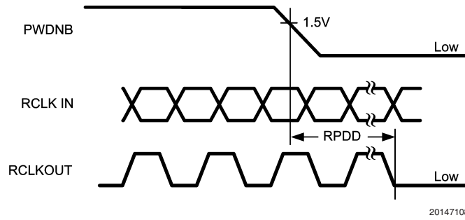
FIGURE 7. Powerdown Delay
