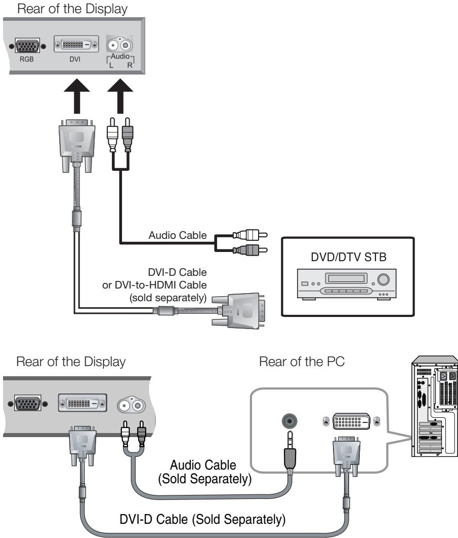
Figure 3-2. DVI Connections
