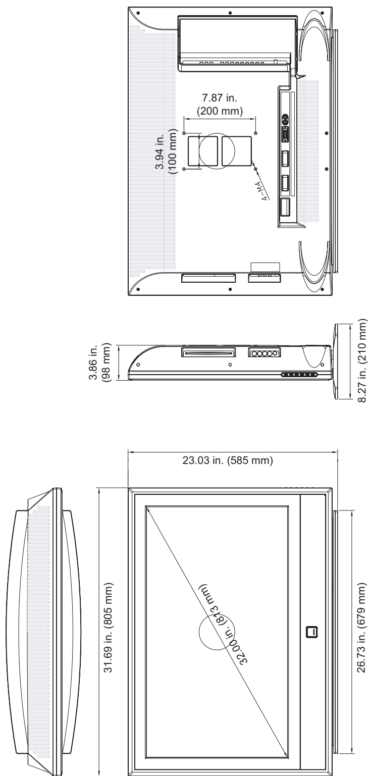
Figure 7-2. CR-32HDi Dimensions
