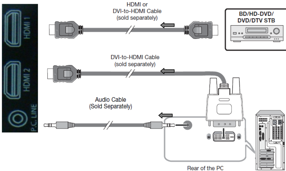
Figure 3-1. HDMI Connections
