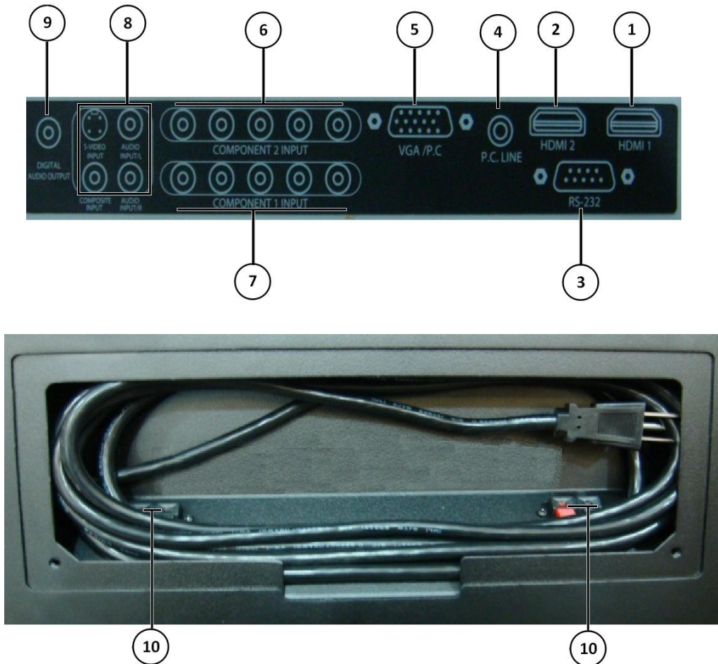
Figure 2-2. Climate Series LCD Input/Output Interfaces
