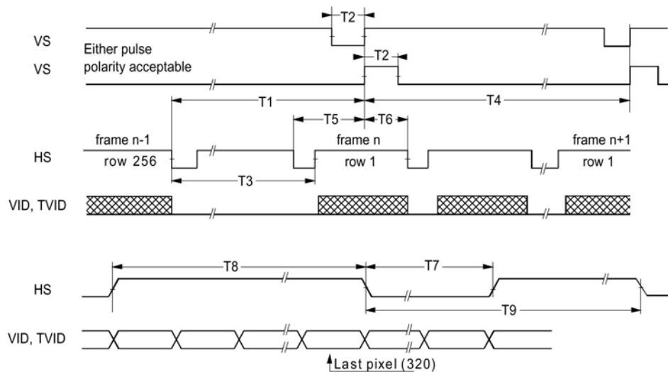
Figure 3. Timing Characteristics
