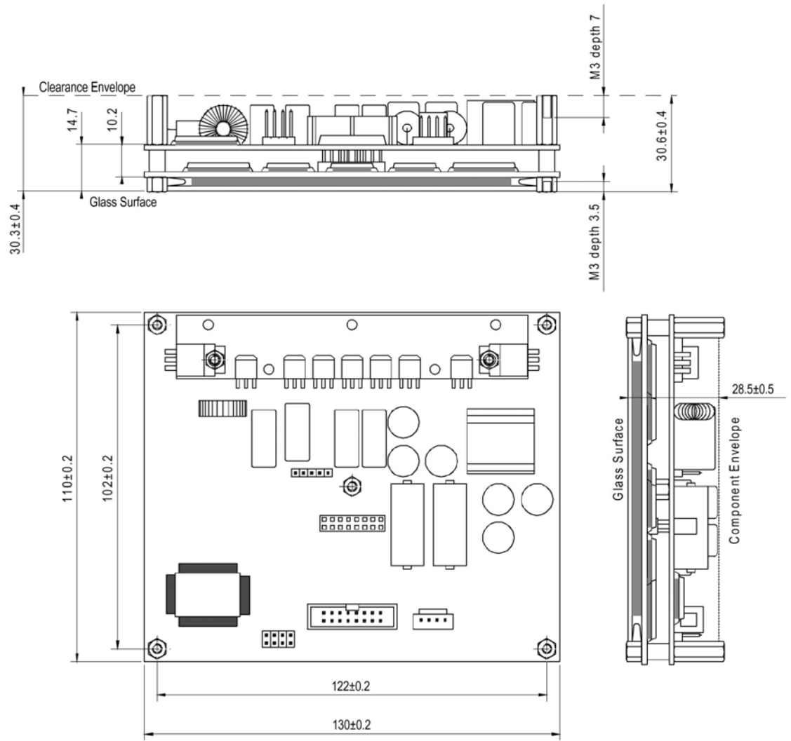
Fig 6. Mechanical dimensions in mm.
