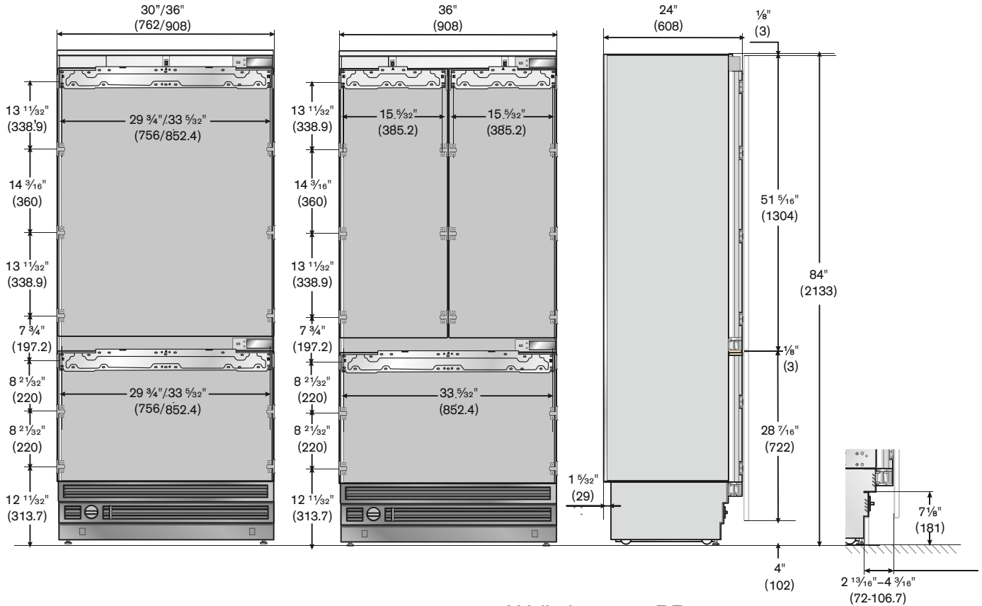
Wall clearance RB/RY 492
