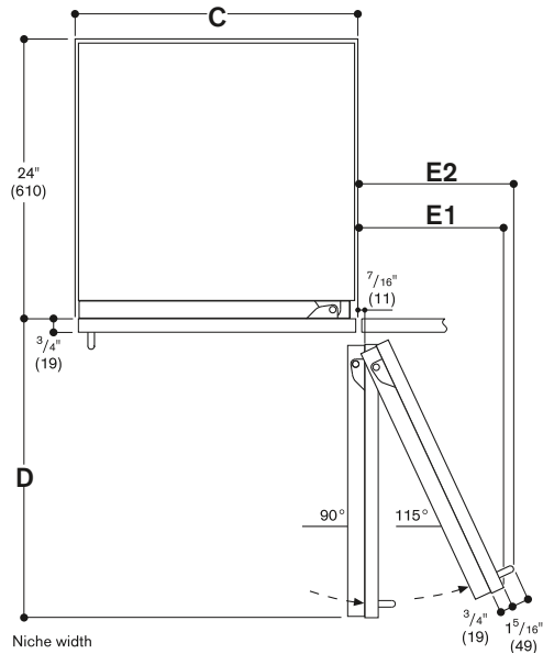
Wall clearance RB 472
