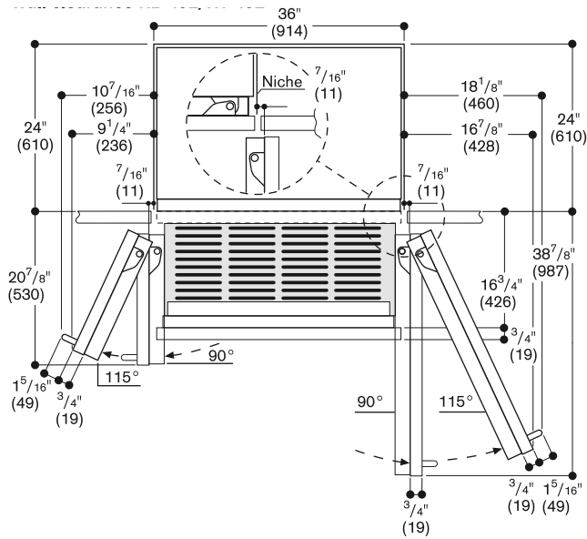
Wall clearance RB/RY 492
