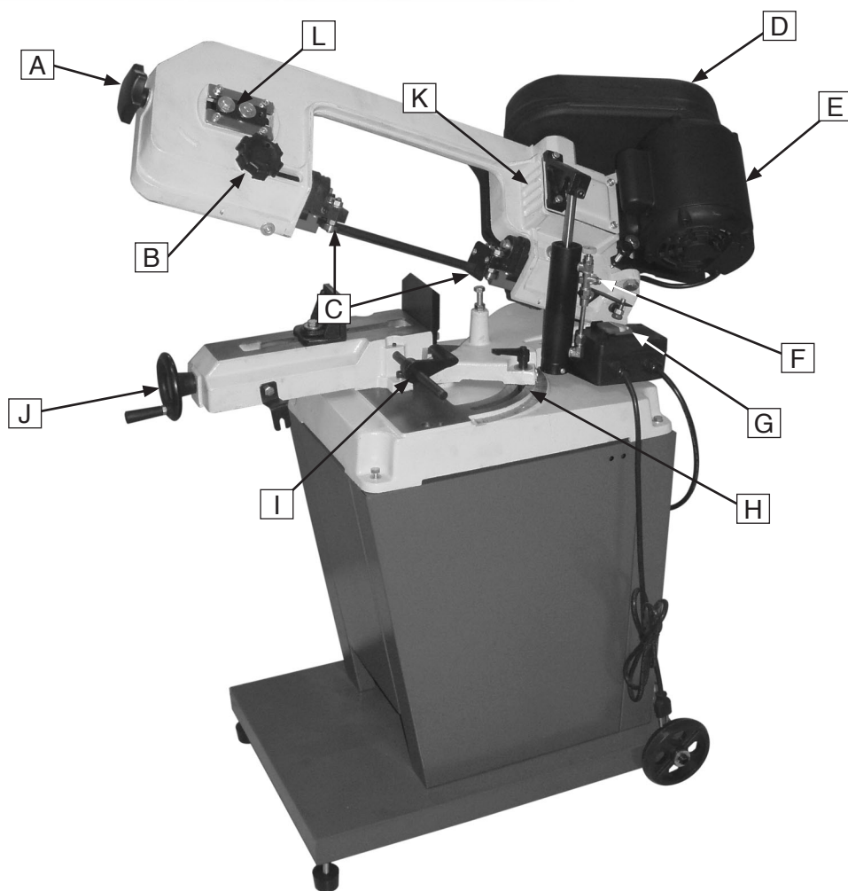
Figure 1. The Model G9742.
