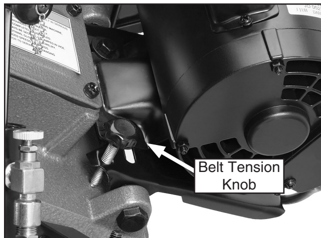
Figure 18. Belt tension knob.
