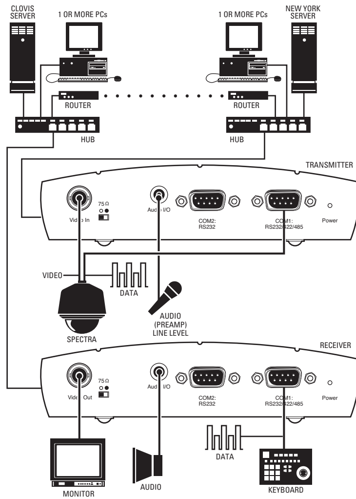
Figure 11. WAN Box-To-Box Connection (Transmitter, Receiver, Spectra)
