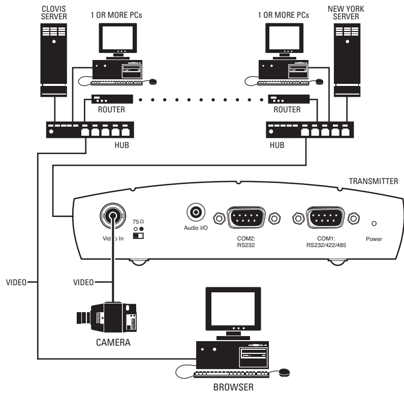
Figure 13. WAN Browser-To-Box Connection (Transmitter, Browser, Fixed Camera)
