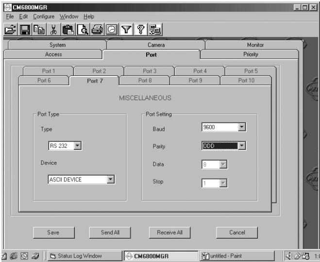
Figure 61. Manager Screen
