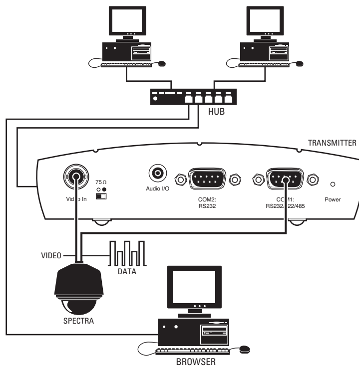
Figure 8. LAN Browser-To-Box Connection (Transmitter, Browser, Spectra)
