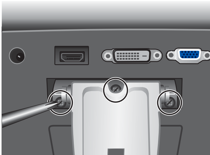
Figure 3-12 Removing the Hinge Screws
