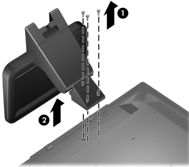
Figure 3-6 Removing the Pedestal Base
