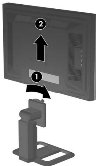
Figure 3-12 Removing the Monitor from the Pedestal Base
