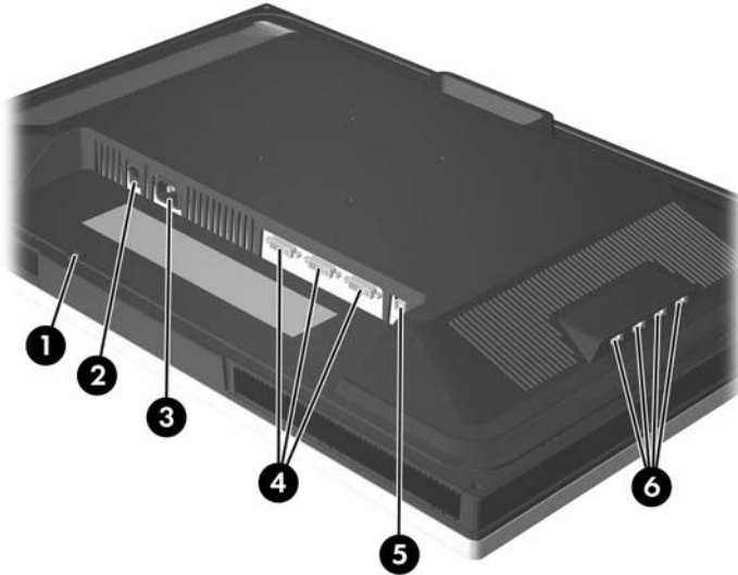
Figure 3-2 Rear Components
