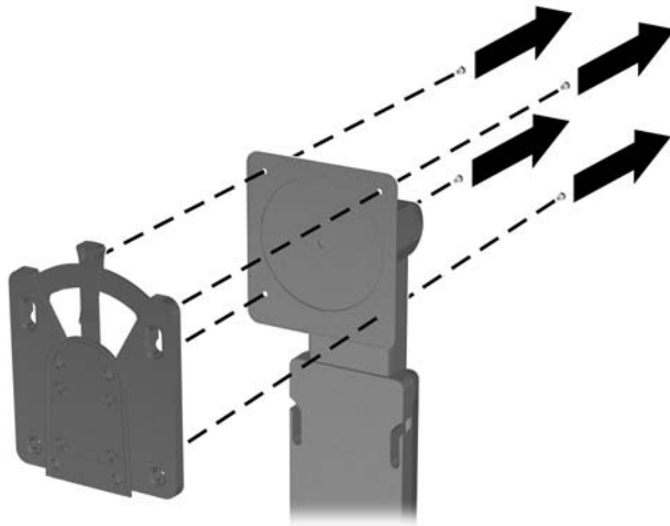
Figure 3-13 Removing the HP Quick Release from the Pedestal Base
