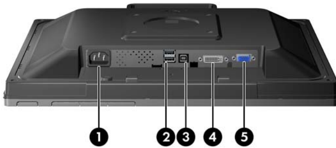
Figure 3-3 Rear Components
