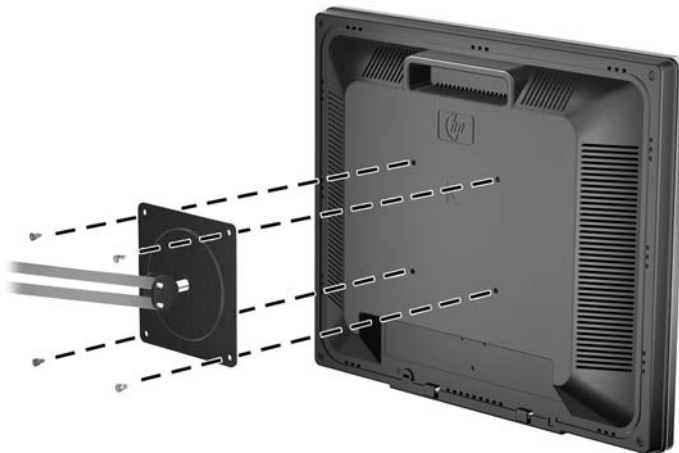
Figure 3-7 Installing the Monitor on a Swing Arm
