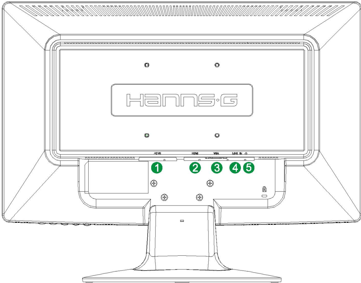
Figure.3. Connecting to a PC (HH221H)
