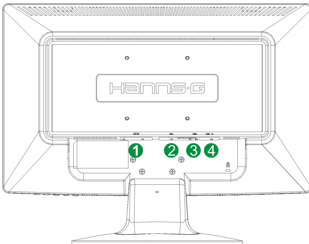
Figure.2. Connecting to a PC (HH221D)
