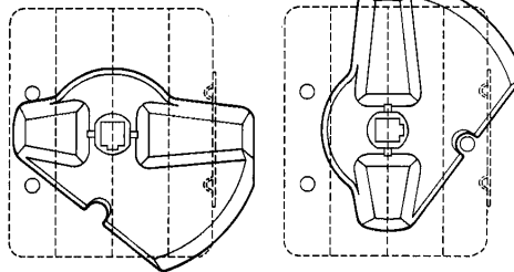
CLOSED POSITION
