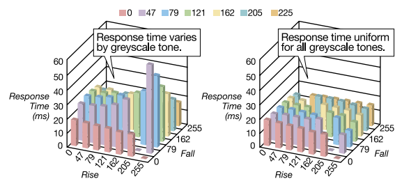
Without Overdrive Circuit (Standard Monitor) With Overdrive Circuit (L778/L578) Response time as measured by EIZO.
