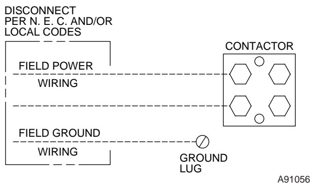
Fig. 9—Line Power Connections
