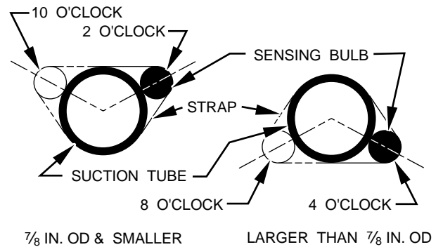
Fig. 5—Position of Sensing Bulb
