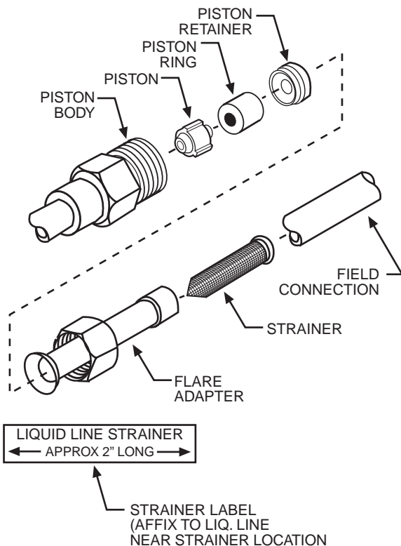
Fig. 4—Check-Flo-Rater® Components (550A, 552A, 591B Only)
