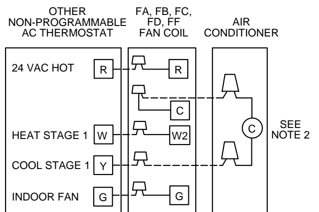
Fig. 10—Typical 24v Circuit Connections
