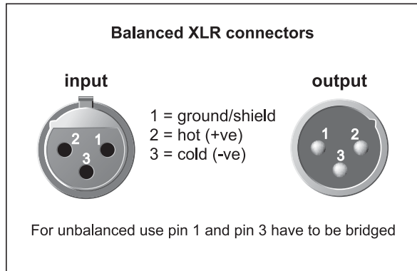
Fig. 4.3: XLR connectors
