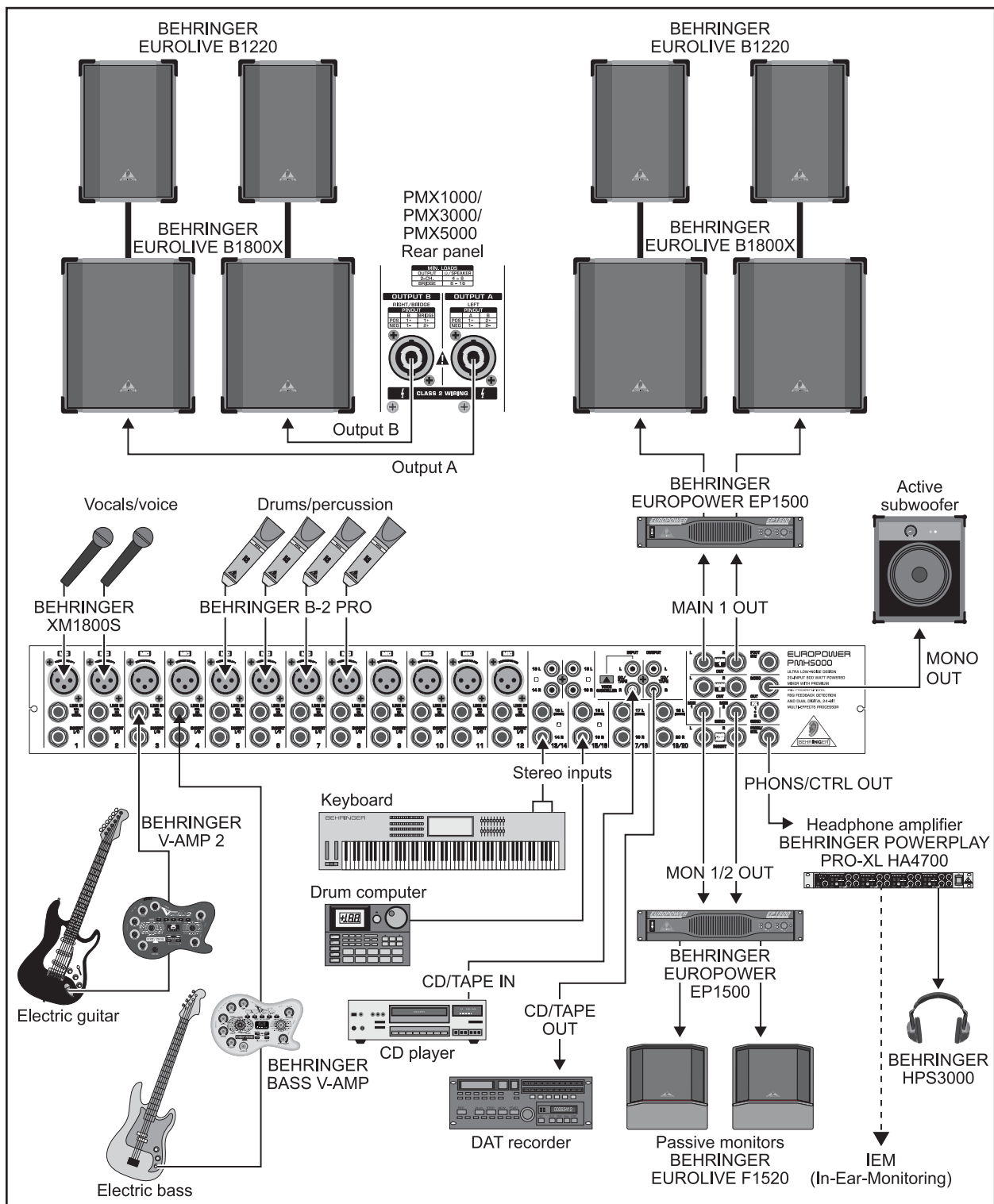
Fig. 5.5: Expanded set-up
