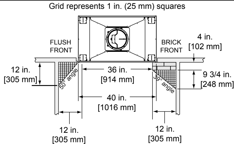
Figure 6.3 Mantel Leg or Wall Projections (Acceptable on both sides of opening)
