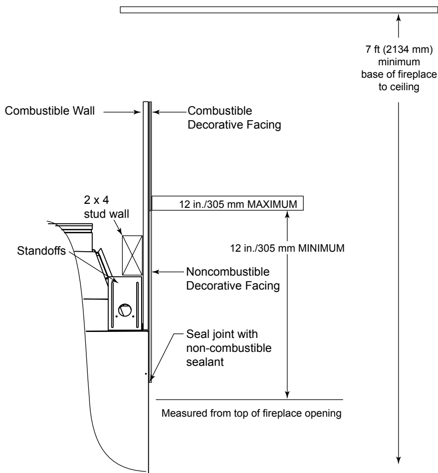
→ Figure 11.4 Clearances to Mantels or other Combustibles above Fireplace
