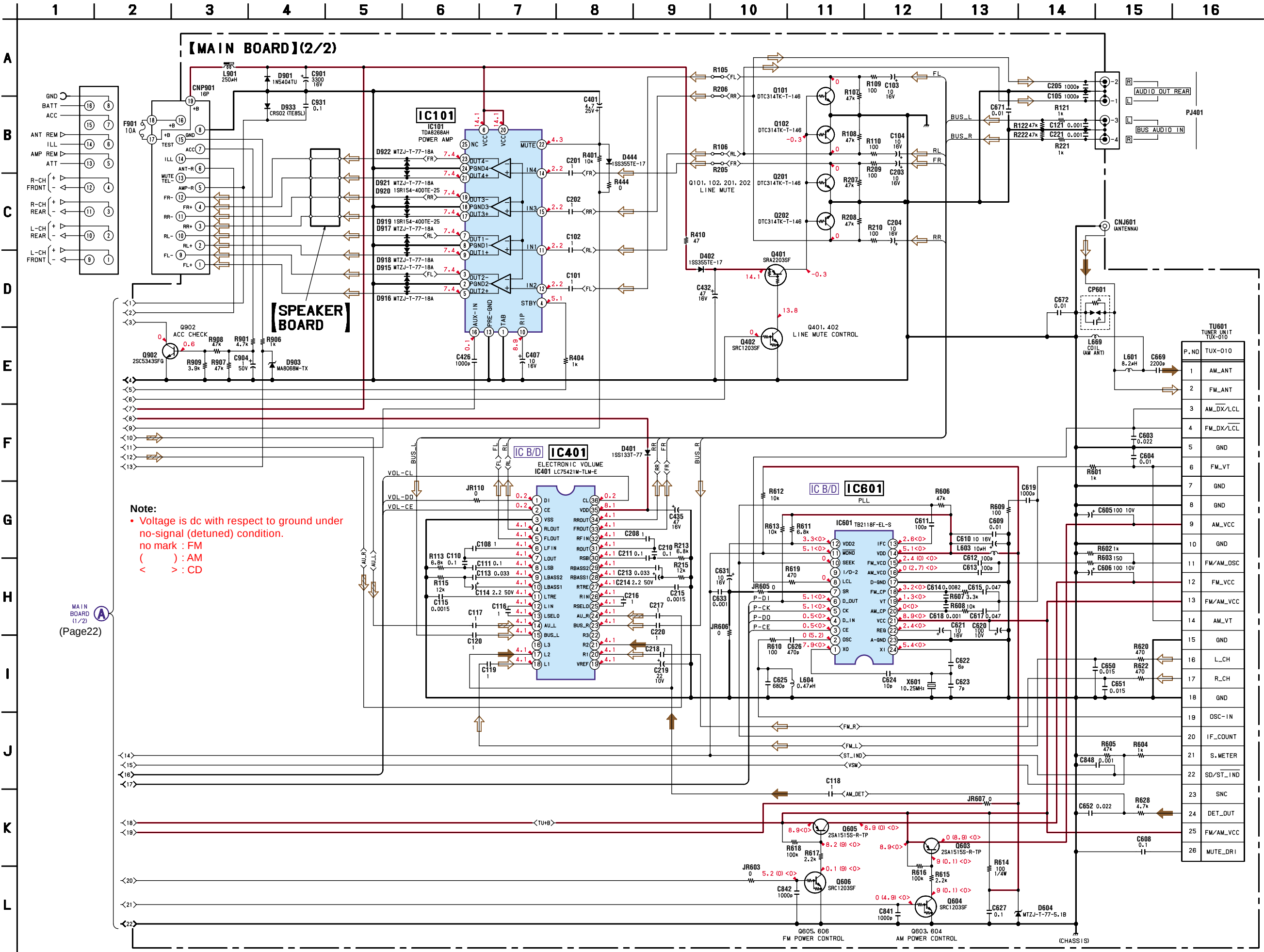
3-10. SCHEMATIC DIAGRAM — MAIN SECTION (2/2) — • Refer to page 26 for IC Block Diagrams.
