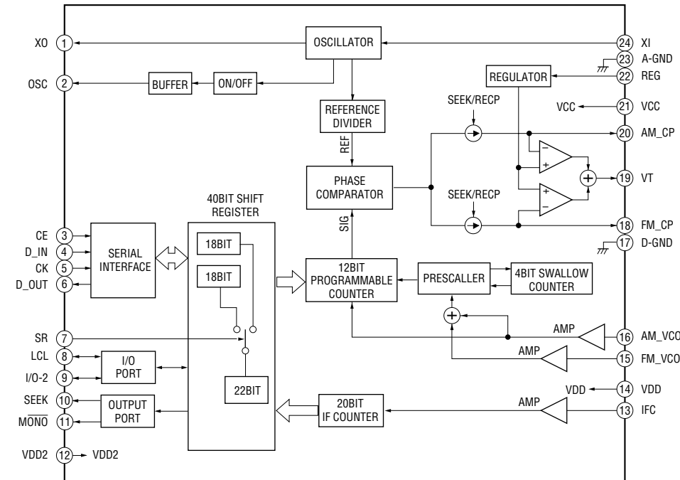
IC601 TB2118F-EL-S
