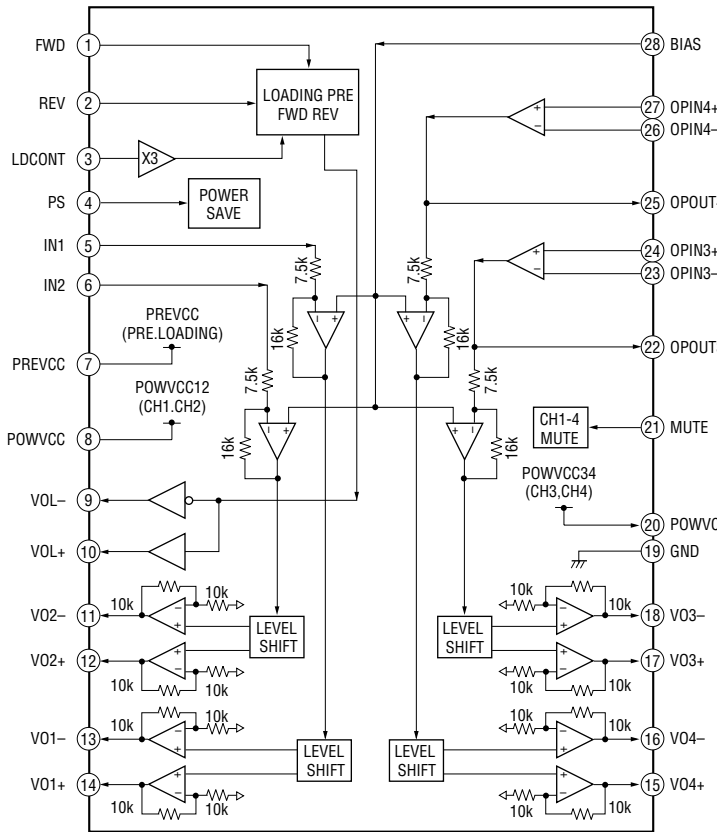
IC2 BA5810FP-E2
