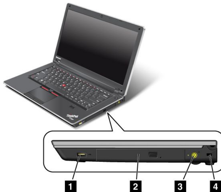
Figure 3. ThinkPad Edge E425 and E525 right-side view
