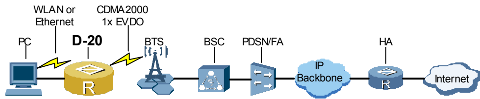
Figure 1-1 The position of D-20 in the 3G network
