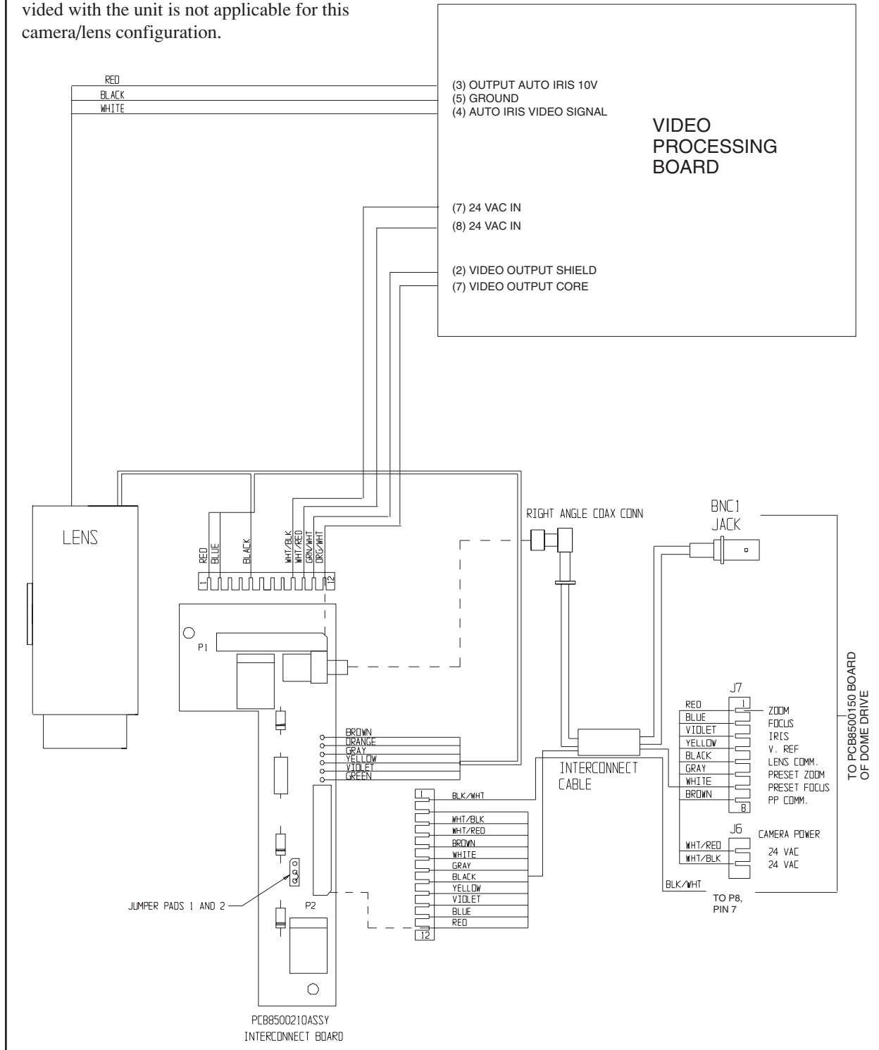
Figure 1. Schematic Diagram for Color Camera/Lens with Manual Iris Override (Model IOP08C3J-1)
