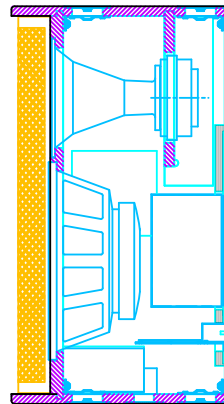
SECTION VIEW
