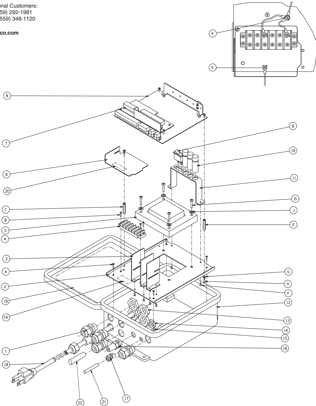
Figure 1. ERD97P21-U Exploded Assembly Diagram
