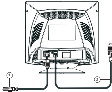
Figure 2 Connecting Cables
