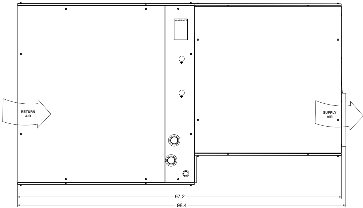
Unit Dimensions ND600 Airhandler & M1CZ600 Evaporator Coil
