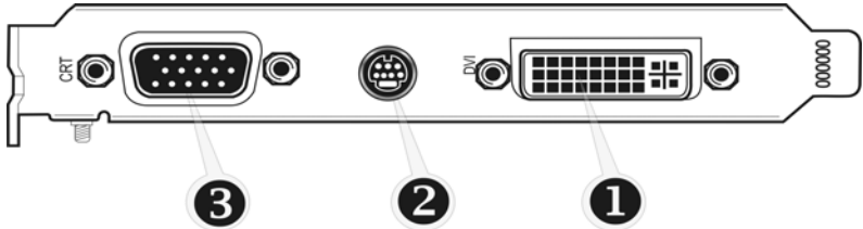
Sample 1: ATI Radeon™ HD 2600 Series Connections
