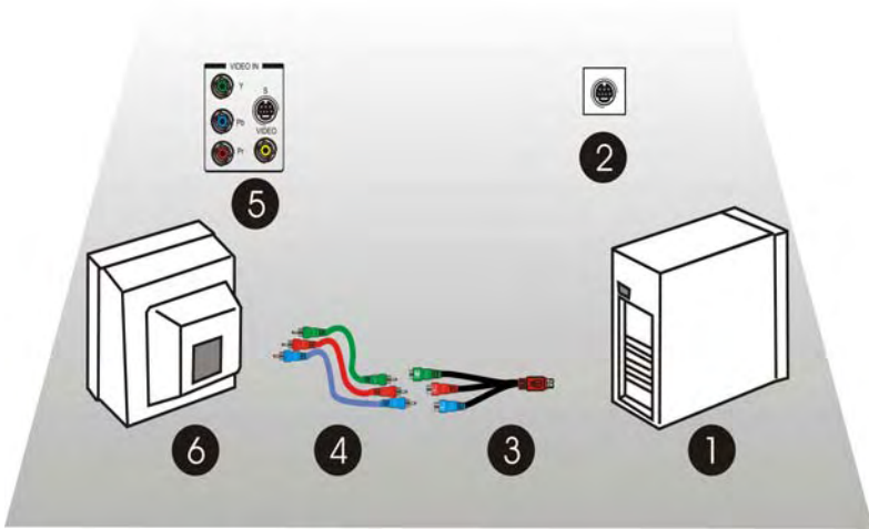
S-Video to Component Video (using the ATI 9-Pin HDTV Output Cable)
