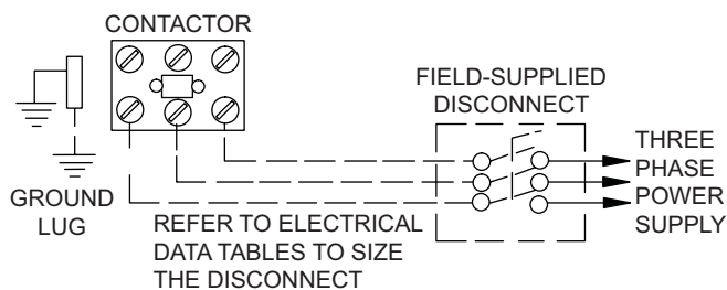
FIGURE 4 - TYPICAL FIELD POWER WIRING DIAGRAM
