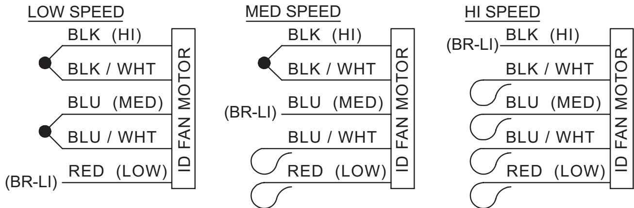
FIGURE 19 - WIRING DIAGRAM DETAIL A (460-3-60 POWER SUPPLY) 1
