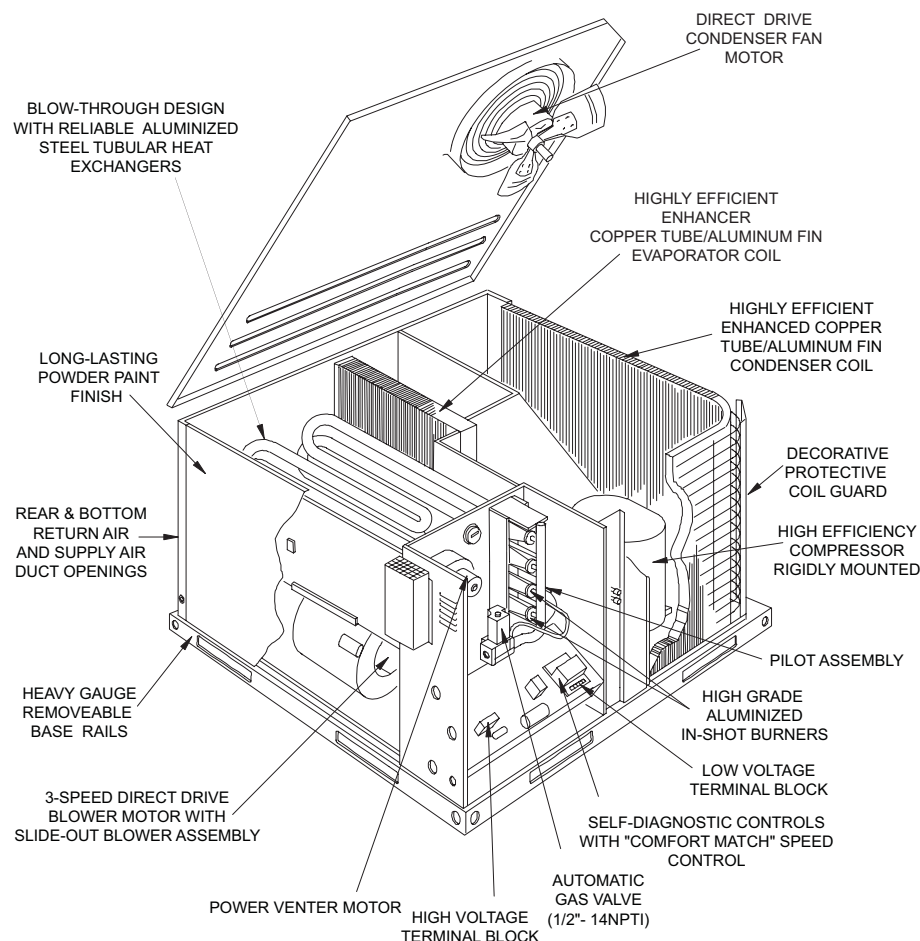
FIGURE 2 - UNIT COMPONENT LOCATION
