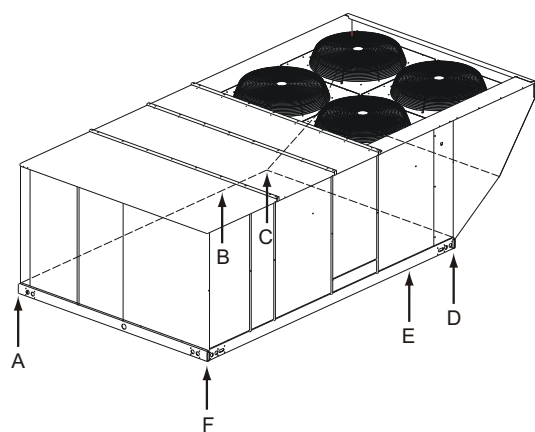
ZJ/ZR Unit 6 Point Load Weight
