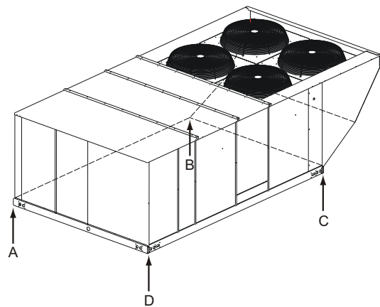
ZJ/ZR Unit 4 Point Load Weight
