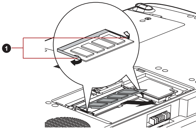
1. Latches
