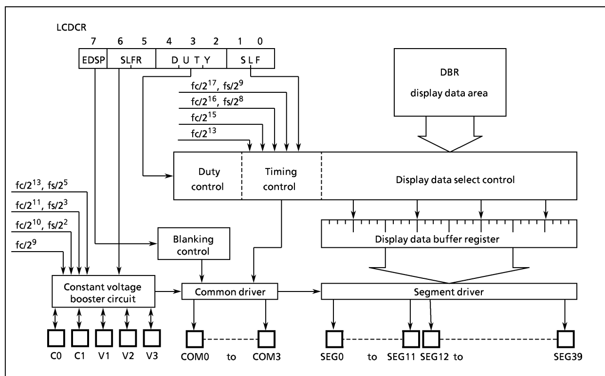
Figure 2-43. LCD Driver
