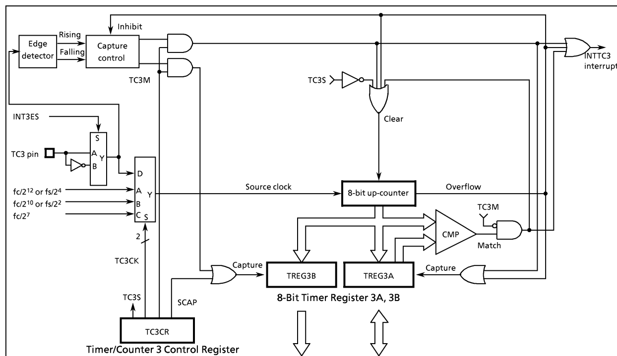
Figure 2-26. Timer/Counter 3
