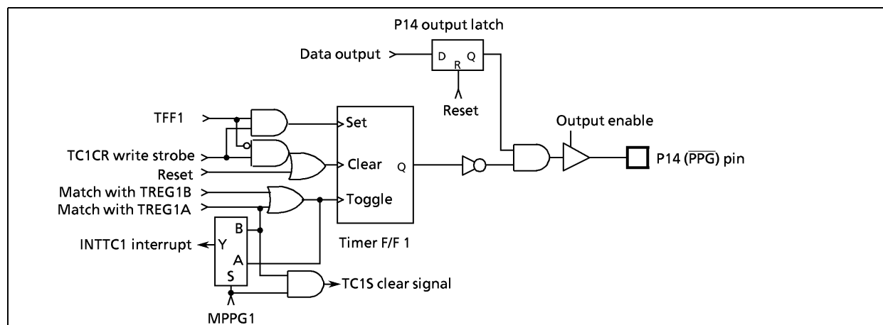
Figure 2-22. PPG Output
