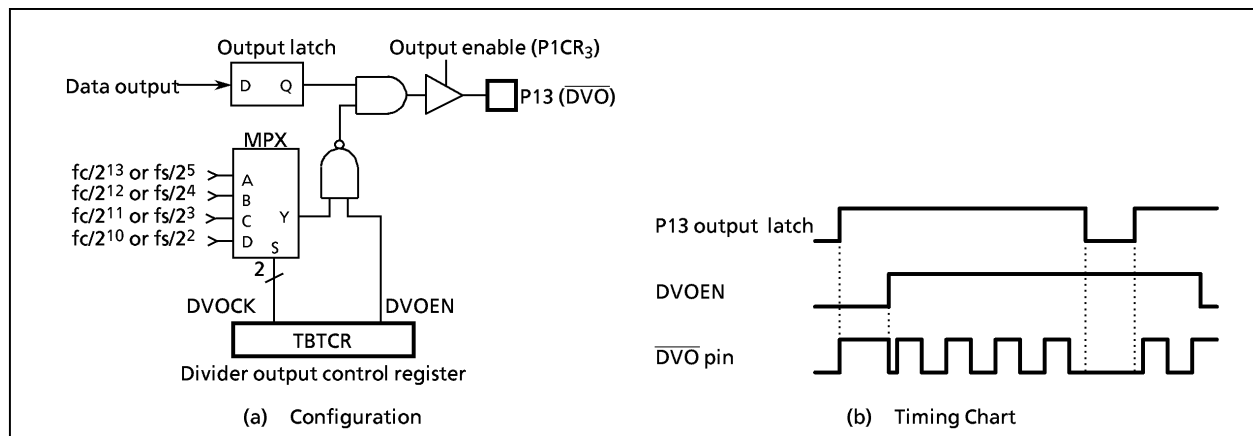
Figure 2-13. Divider Output
