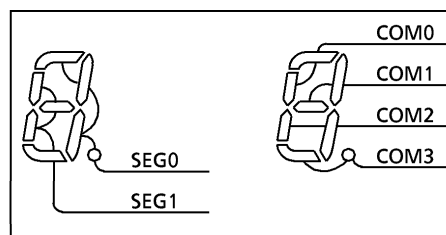
Figure 2-50. Example of COM, SEG Pin Connection (1/4 Duty)
