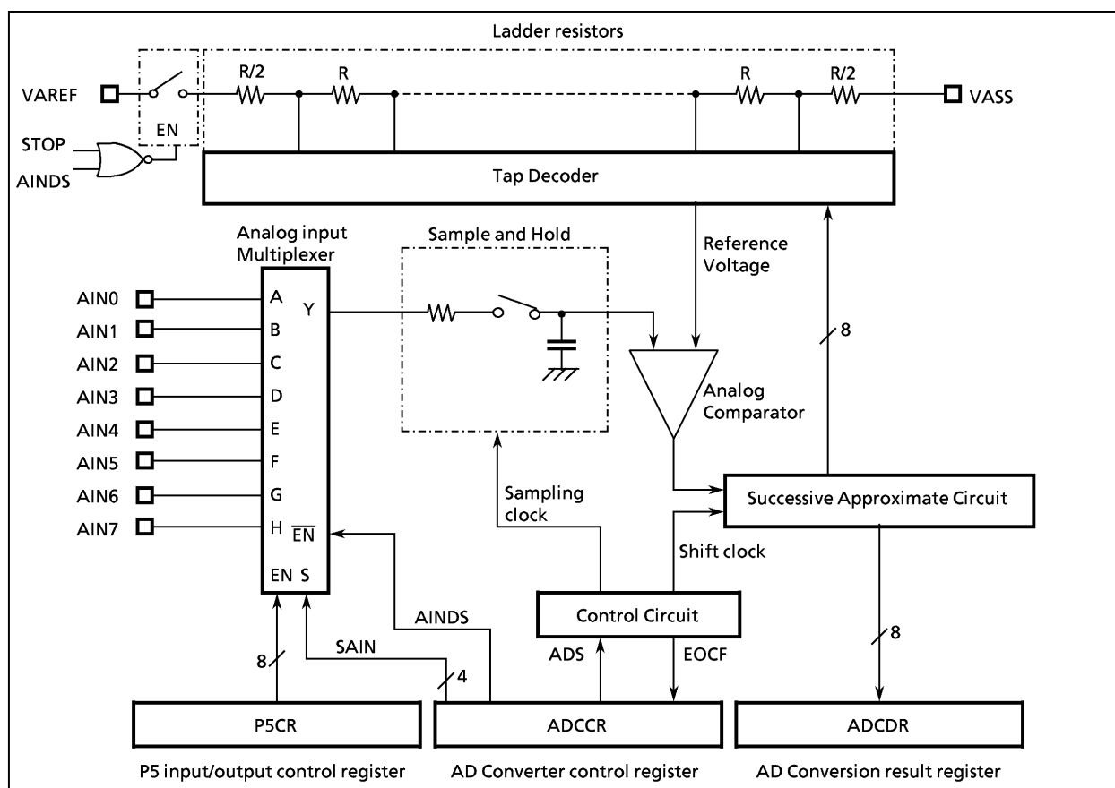
Figure 2-58. AD Converter
