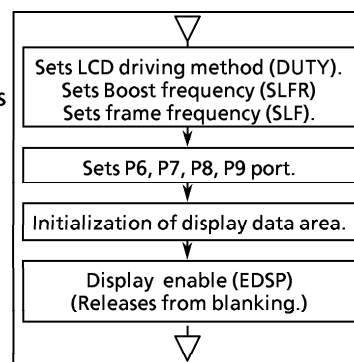
Figure 2-49. Initial Setting of LCD Driver
