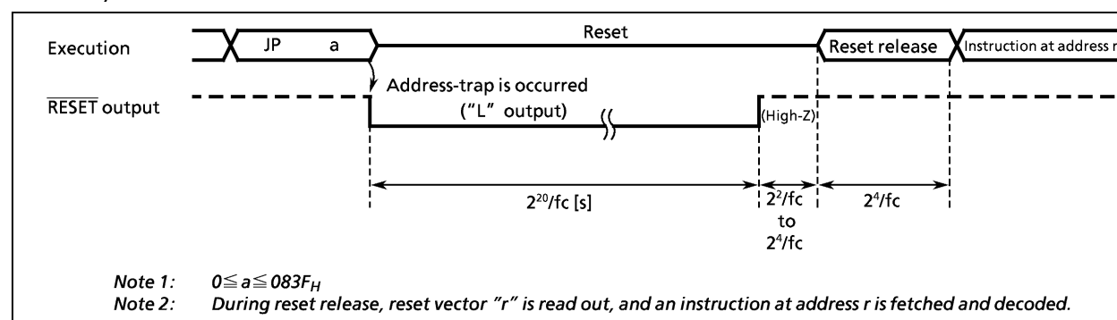
Figure 1-31. Address-Trap-Reset
