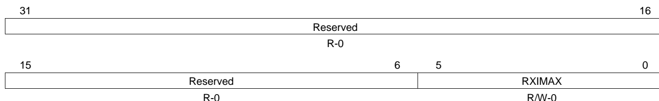
Figure 25. EMAC Control Module Receive Interrupts per Millisecond Register (CMRXINTMAX)
