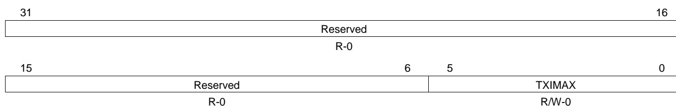
Figure 26. EMAC Control Module Transmit Interrupts per Millisecond Register (CMTXINTMAX)
