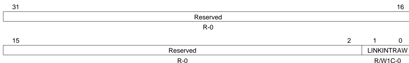
Figure 31. MDIO Link Status Change Interrupt (Unmasked) Register (LINKINTRAW)
