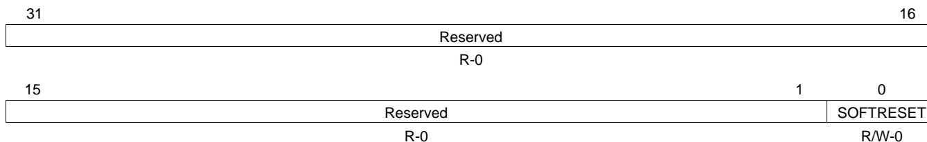
Figure 14. EMAC Control Module Software Reset Register (CMSOFTRESET)
