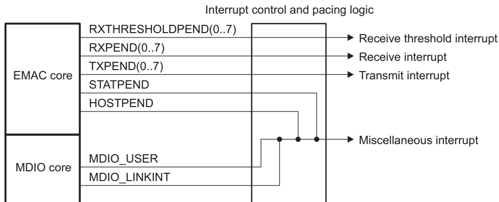
Figure 12. EMAC Control Module Interrupt Logic Diagram
