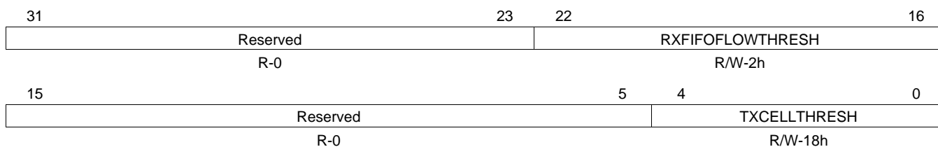
Figure 72. FIFO Control Register (FIFOCONTROL)
