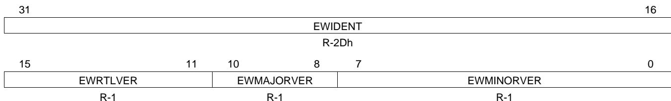
Figure 13. EMAC Control Module Identification and Version Register (CMIDVER)
