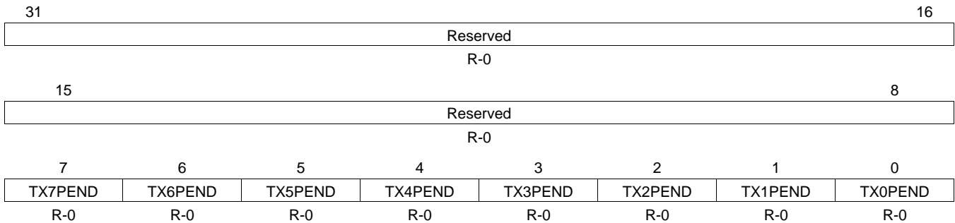
Figure 47. Transmit Interrupt Status (Unmasked) Register (TXINTSTATRAW)
