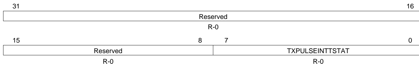
Figure 23. EMAC Control Module Transmit Interrupt Status Register (CMTXINTSTAT)
