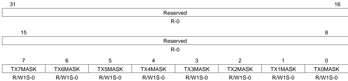
Figure 49. Transmit Interrupt Mask Set Register (TXINTMASKSET)
