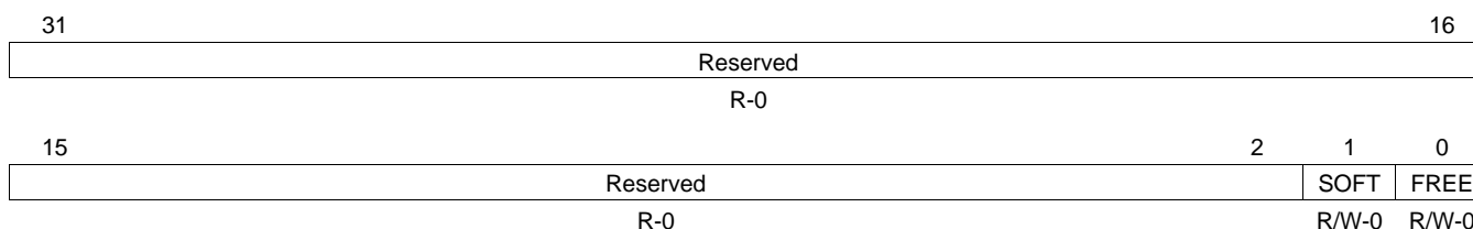
Figure 15. EMAC Control Module Emulation Control Register (CMEMCONTROL)
