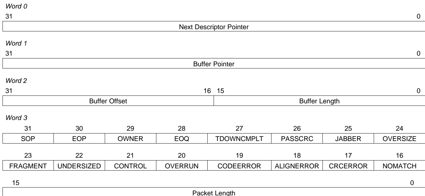
Figure 8. Receive Buffer Descriptor Format
