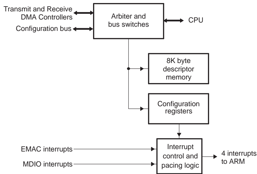
Figure 9. EMAC Control Module Block Diagram
