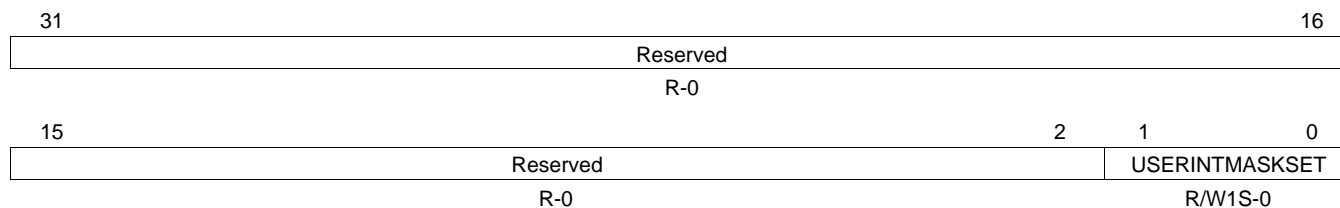
Figure 35. MDIO User Command Complete Interrupt Mask Set Register (USERINTMASKSET)
