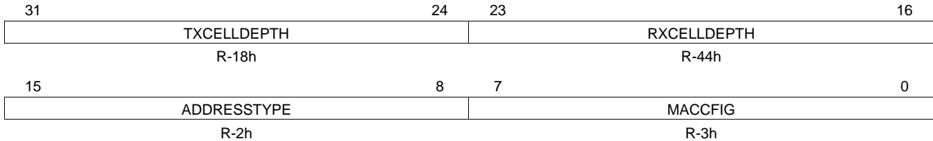
Figure 73. MAC Configuration Register (MACCONFIG)
