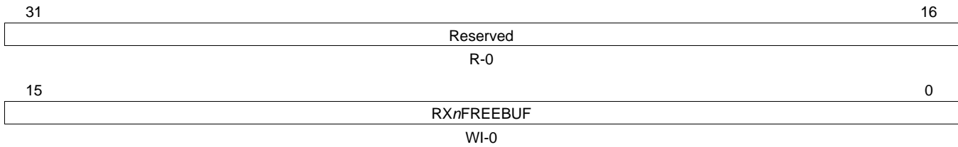
Figure 68. Receive Channel n Free Buffer Count Register (RXnFREEBUFFER)
