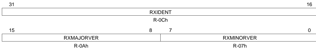
Figure 44. Receive Identification and Version Register (RXIDVER)
