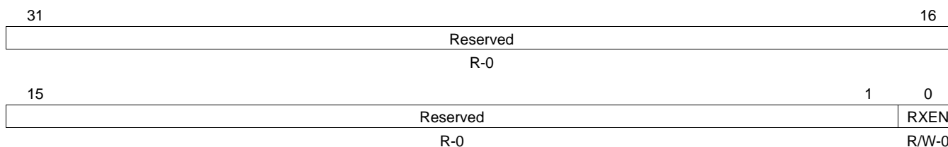
Figure 45. Receive Control Register (RXCONTROL)
