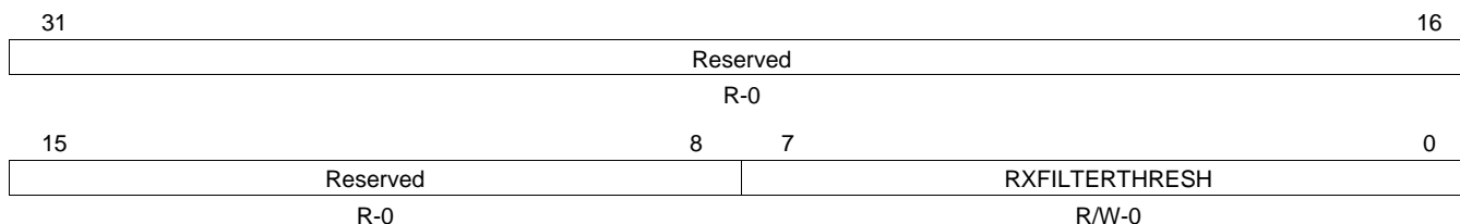
Figure 66. Receive Filter Low Priority Frame Threshold Register (RXFILTERLOWTHRESH)
