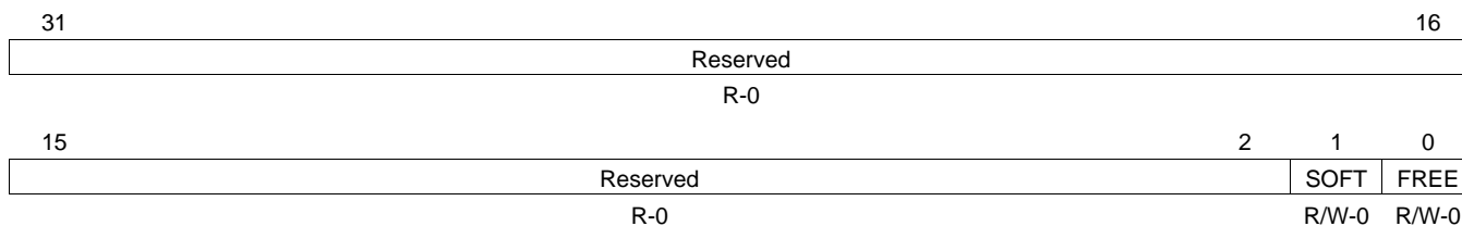
Figure 71. Emulation Control Register (EMCONTROL)
