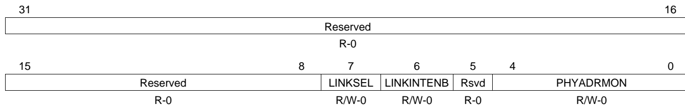
Figure 38. MDIO User PHY Select Register 0 (USERPHYSEL0)
