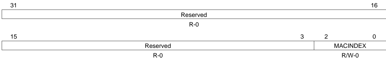
Figure 85. MAC Index Register (MACINDEX)
