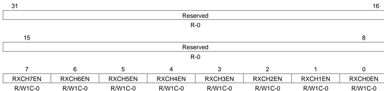
Figure 63. Receive Unicast Clear Register (RXUNICASTCLEAR)
