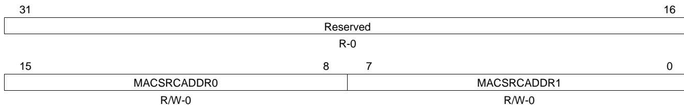
Figure 75. MAC Source Address Low Bytes Register (MACSRCADDRLO)
