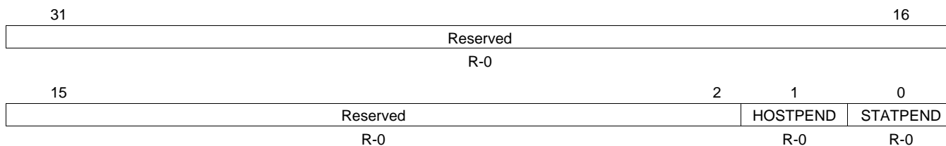
Figure 57. MAC Interrupt Status (Unmasked) Register (MACINTSTATRAW)
