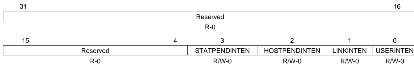
Figure 20. EMAC Control Module Miscellaneous Interrupt Enable Register (CMMISCINTEN)
