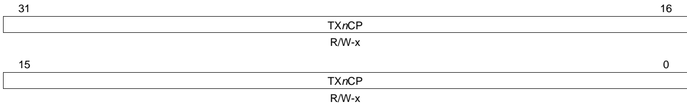
Figure 88. Transmit Channel n Completion Pointer Register (TX n CP)
