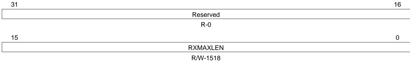
Figure 64. Receive Maximum Length Register (RXMAXLEN)
