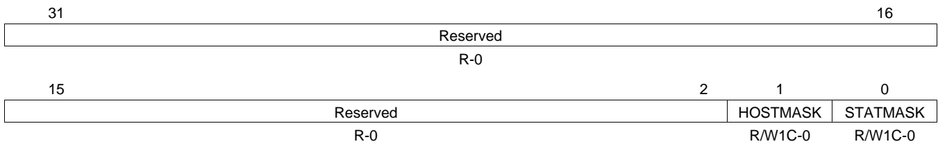
Figure 60. MAC Interrupt Mask Clear Register (MACINTMASKCLEAR)
