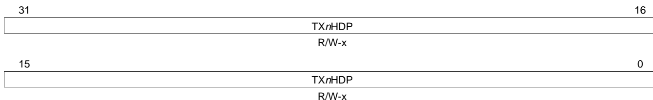
Figure 86. Transmit Channel n DMA Head Descriptor Pointer Register (TXnHDP)
