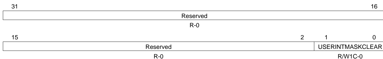
Figure 36. MDIO User Command Complete Interrupt Mask Clear Register (USERINTMASKCLEAR)
