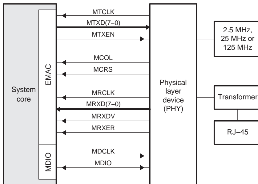
Figure 2. Ethernet Configuration—MII Connections
