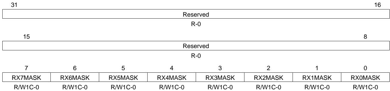
Figure 56. Receive Interrupt Mask Clear Register (RXINTMASKCLEAR)
