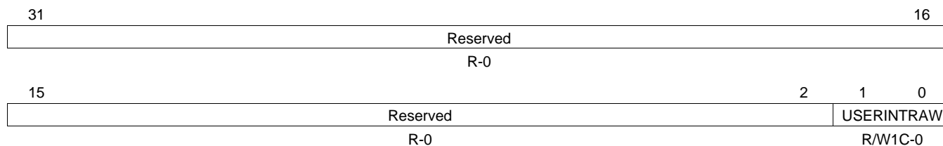
Figure 33. MDIO User Command Complete Interrupt (Unmasked) Register (USERINTRAW)
