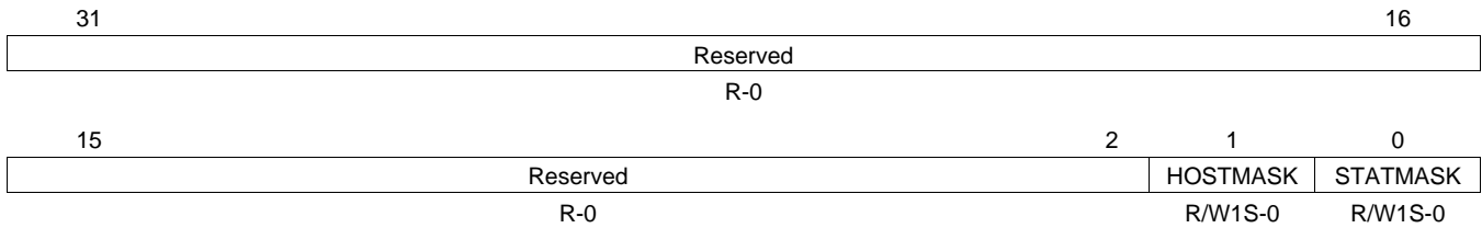
Figure 59. MAC Interrupt Mask Set Register (MACINTMASKSET)
