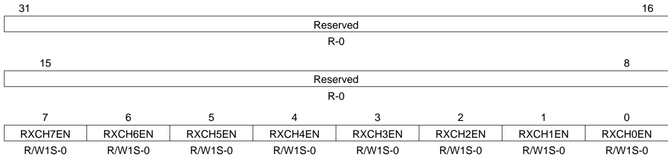
Figure 62. Receive Unicast Enable Set Register (RXUNICASTSET)
