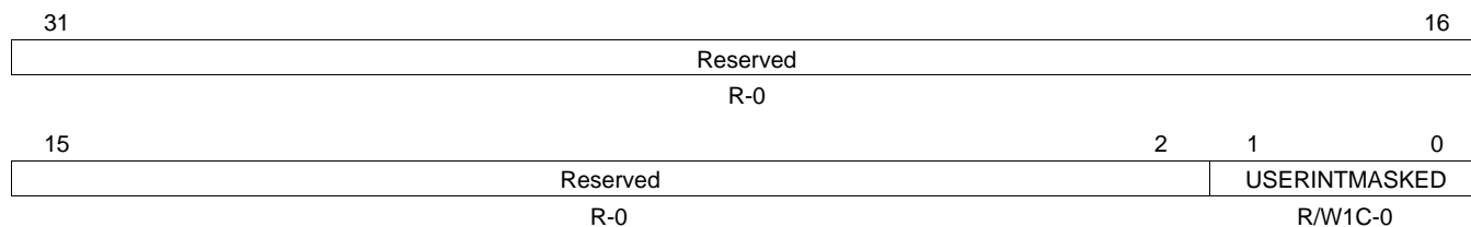
Figure 34. MDIO User Command Complete Interrupt (Masked) Register (USERINTMASKED)
