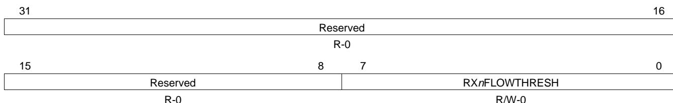
Figure 67. Receive Channel n Flow Control Threshold Register (RXnFLOWTHRESH)
