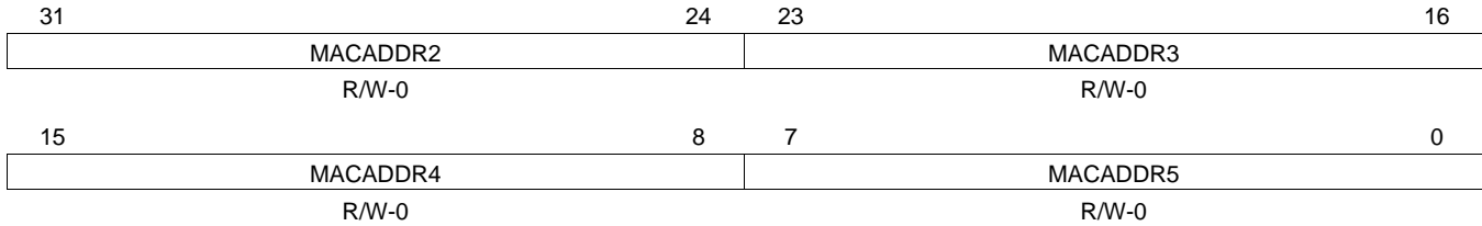
Figure 84. MAC Address High Bytes Register (MACADDRHI)
