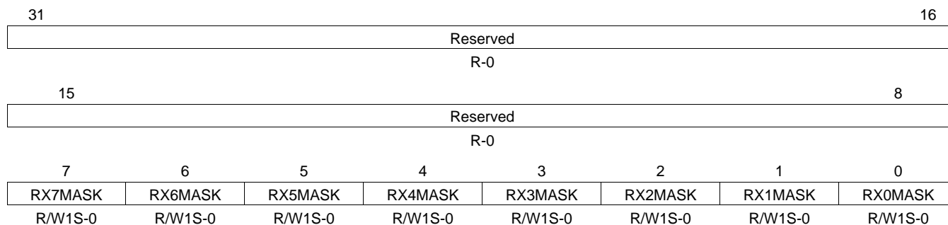
Figure 55. Receive Interrupt Mask Set Register (RXINTMASKSET)
