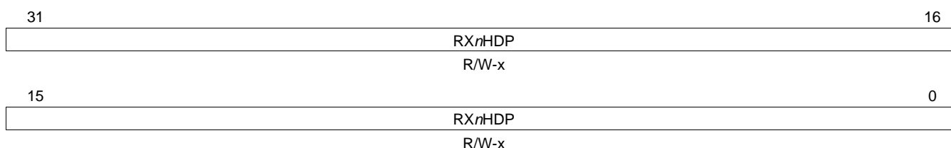
Figure 87. Receive Channel n DMA Head Descriptor Pointer Register (RXnHDP)
