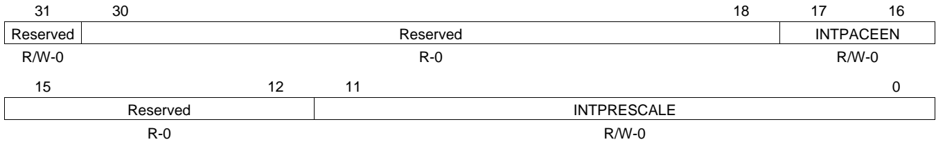
Figure 16. EMAC Control Module Interrupt Control Register (CMINTCTRL)
