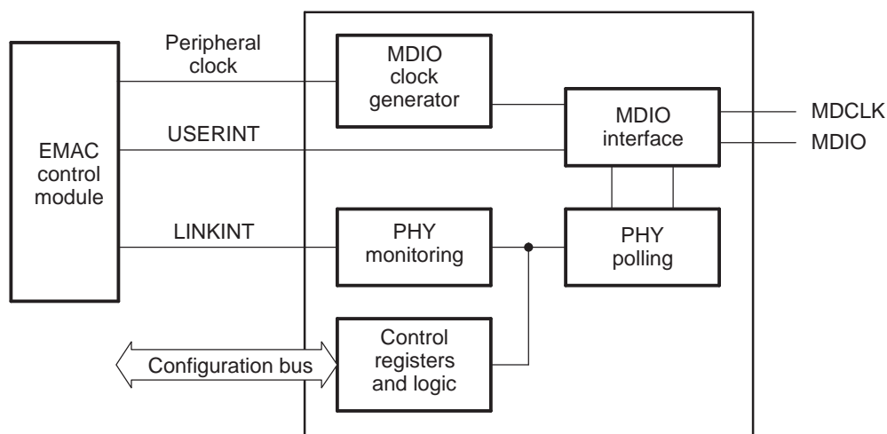
Figure 10. MDIO Module Block Diagram
