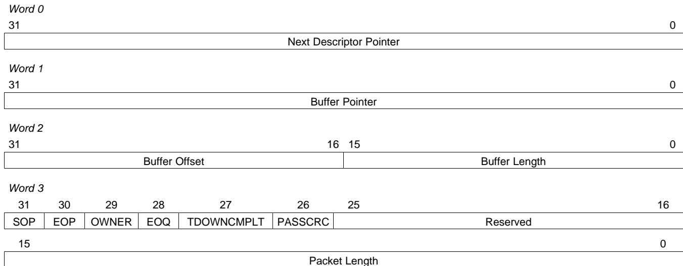
Figure 7. Transmit Buffer Descriptor Format
