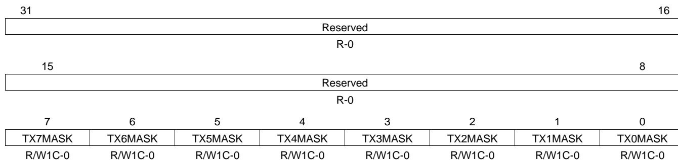
Figure 50. Transmit Interrupt Mask Clear Register (TXINTMASKCLEAR)
