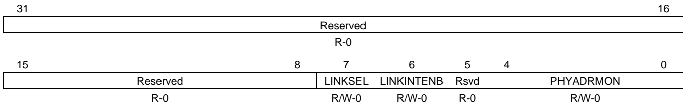
Figure 40. MDIO User PHY Select Register 1 (USERPHYSEL1)
