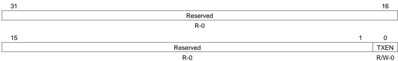
Figure 42. Transmit Control Register (TXCONTROL)
