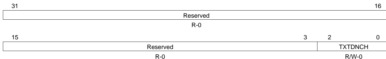
Figure 43. Transmit Teardown Register (TXTEARDOWN)
