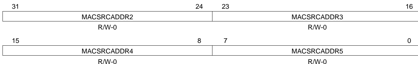
Figure 76. MAC Source Address High Bytes Register (MACSRCADDRHI)
