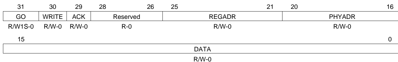
Figure 37. MDIO User Access Register 0 (USERACCESS0)
