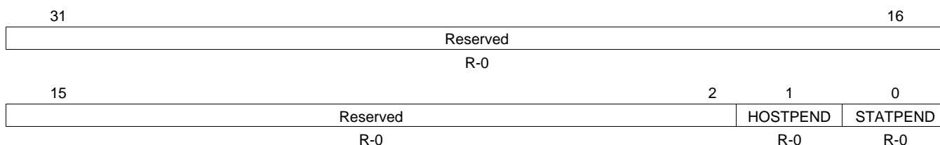
Figure 58. MAC Interrupt Status (Masked) Register (MACINTSTATMASKED)
