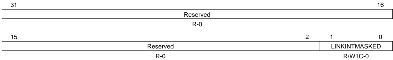
Figure 32. MDIO Link Status Change Interrupt (Masked) Register (LINKINTMASKED)
