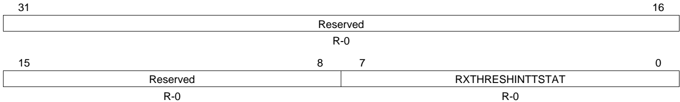
Figure 21. EMAC Control Module Receive Threshold Interrupt Status Register (CMRXTHRESHINTSTAT)
