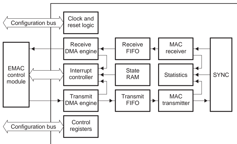
Figure 11. EMAC Module Block Diagram
