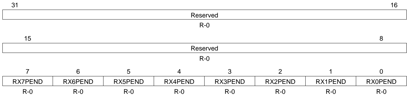
Figure 54. Receive Interrupt Status (Masked) Register (RXINTSTATMASKED)
