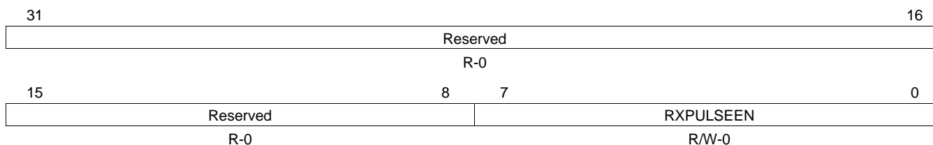
Figure 18. EMAC Control Module Receive Interrupt Enable Register (CMRXINTEN)
