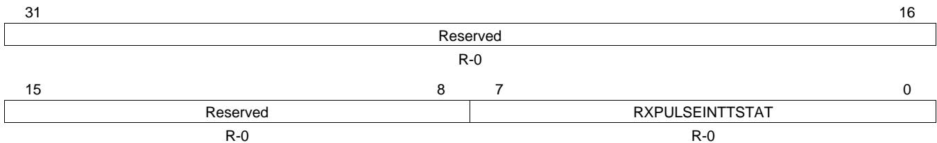
Figure 22. EMAC Control Module Receive Interrupt Status Register (CMRXINTSTAT)
