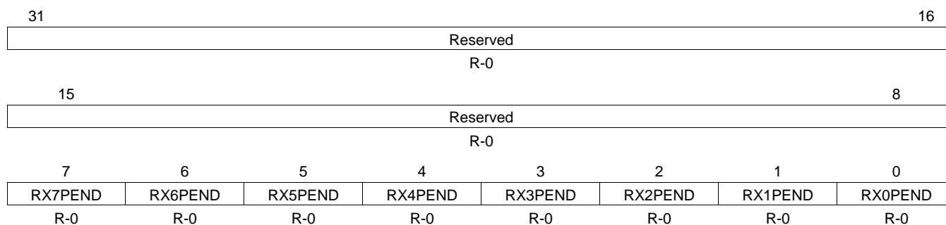
Figure 53. Receive Interrupt Status (Unmasked) Register (RXINTSTATRAW)
