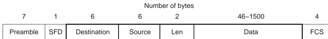
Figure 4. Ethernet Frame Format
