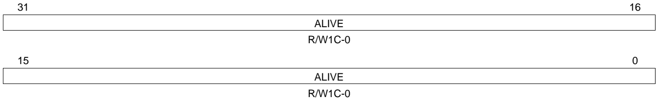
Figure 29. PHY Acknowledge Status Register (ALIVE)
