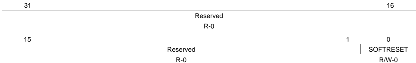
Figure 74. Soft Reset Register (SOFTRESET)
