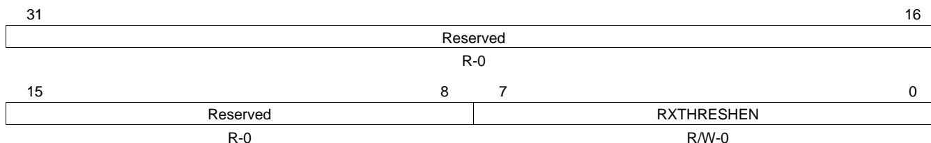
Figure 17. EMAC Control Module Receive Threshold Interrupt Enable Register (CMRXTHRESHINTEN)
