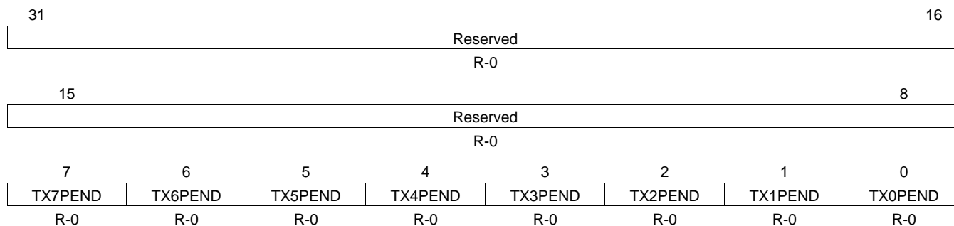
Figure 48. Transmit Interrupt Status (Masked) Register (TXINTSTATMASKED)
