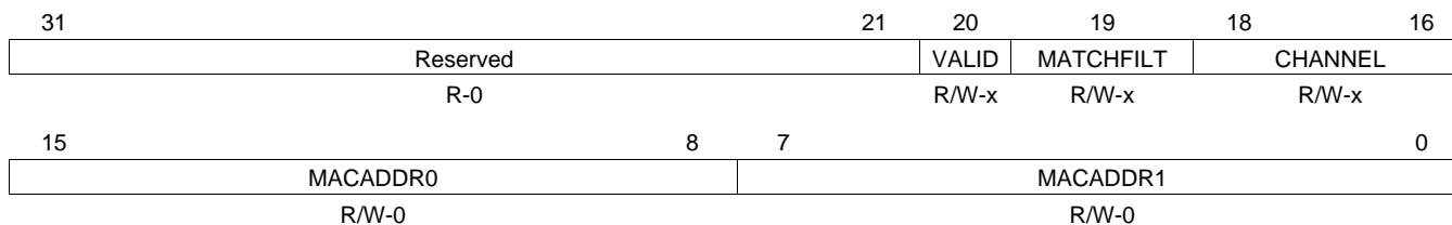
Figure 83. MAC Address Low Bytes Register (MACADDRLO)
