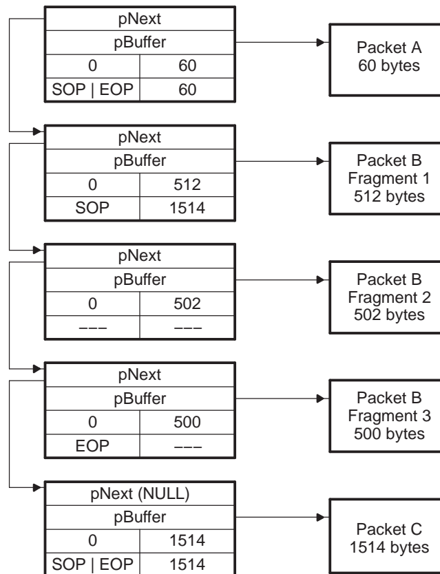
Figure 6. Typical Descriptor Linked List
