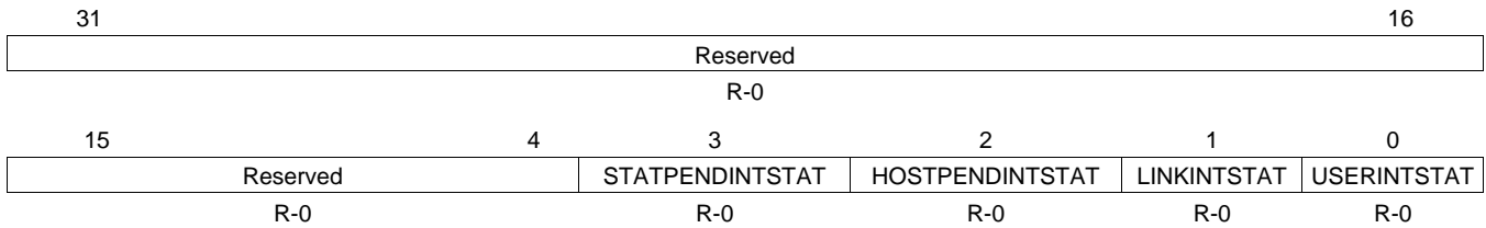
Figure 24. EMAC Control Module Miscellaneous Interrupt Status Register (CMMISCINTSTAT)
