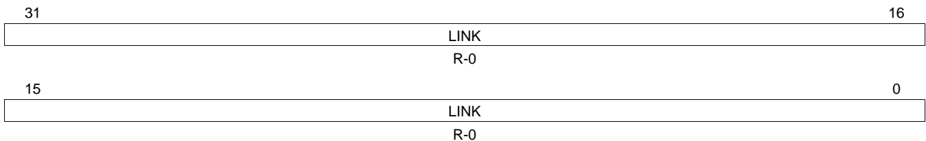
Figure 30. PHY Link Status Register (LINK)
