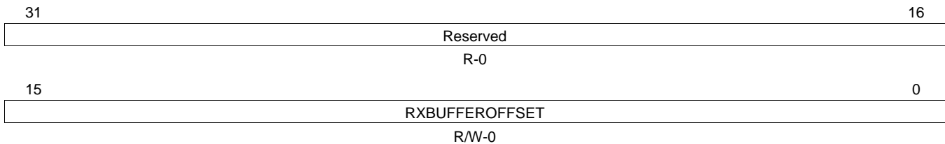
Figure 65. Receive Buffer Offset Register (RXBUFFEROFFSET)
