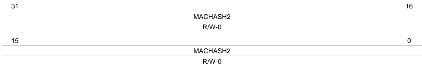
Figure 78. MAC Hash Address Register 2 (MACHASH2)
