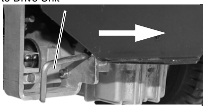
Transmission Bypass Lever Engaged to Push Unit Manually
