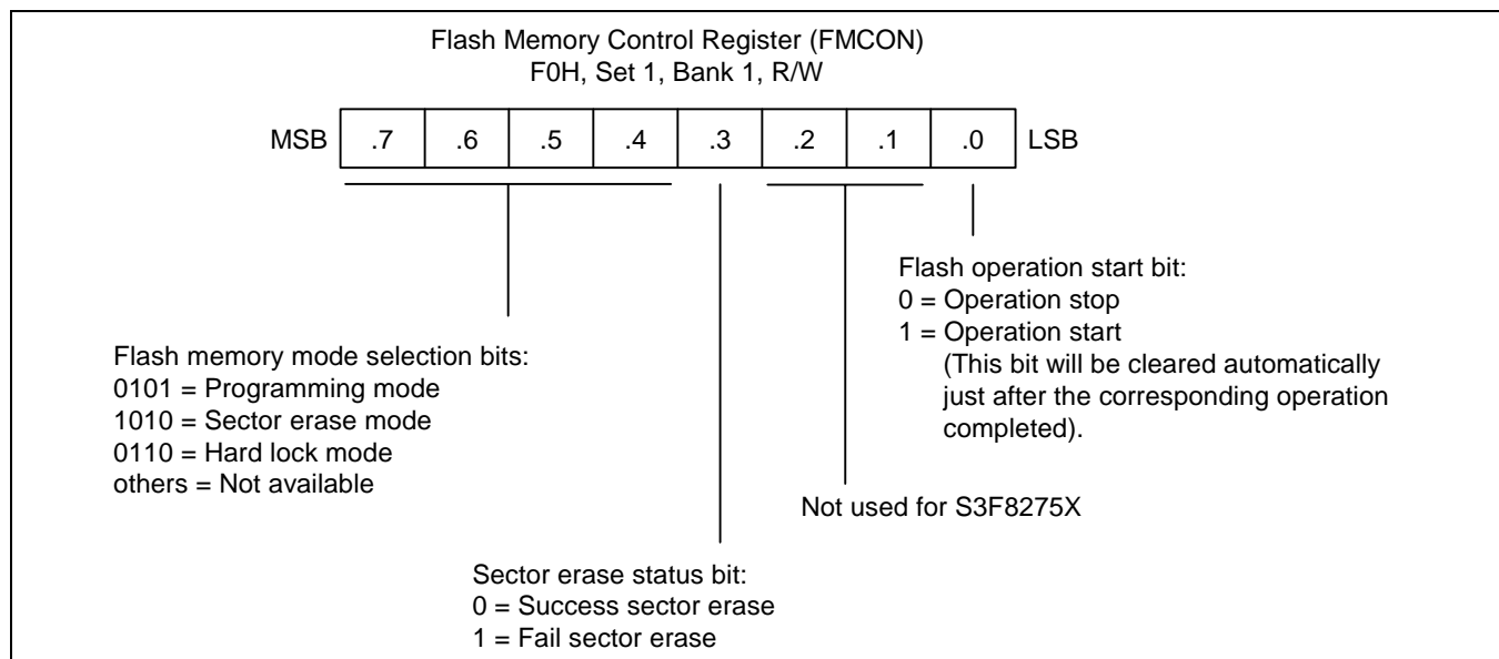
Figure 16-1. Flash Memory Control Register (FMCON)
