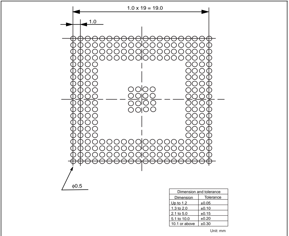
Figure 6 Recommended Dimensions for Mount Pad
