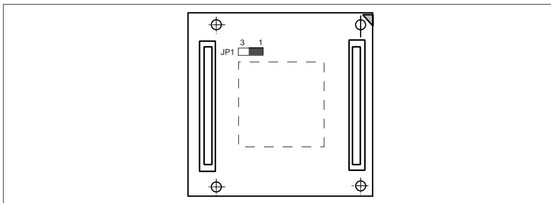
Figure 11 JP1 Jumper
