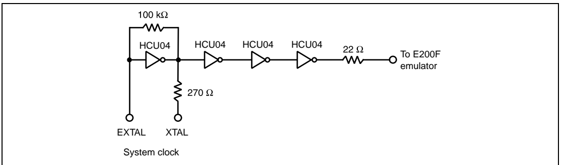
Figure 10 Clock Oscillator
