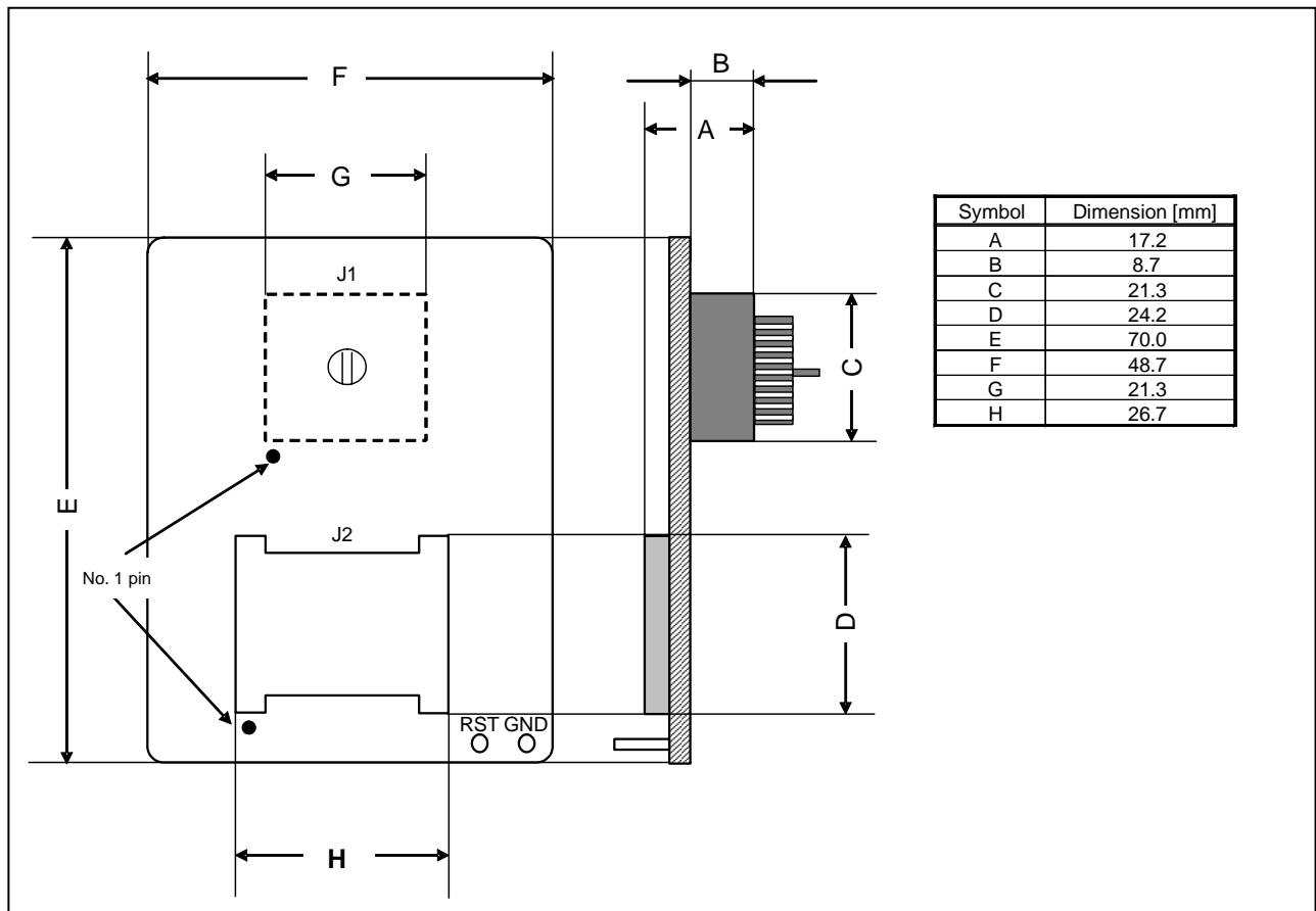
Figure 6 External dimensions of the M38C29T-64LCA
