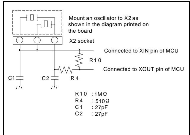
Figure 6.1 Connection diagram of X2 socket
