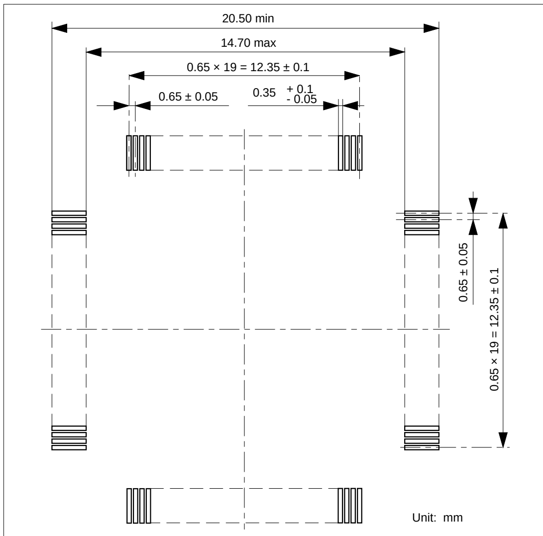
Figure 4 Recommended Dimensions for Mount Pad
