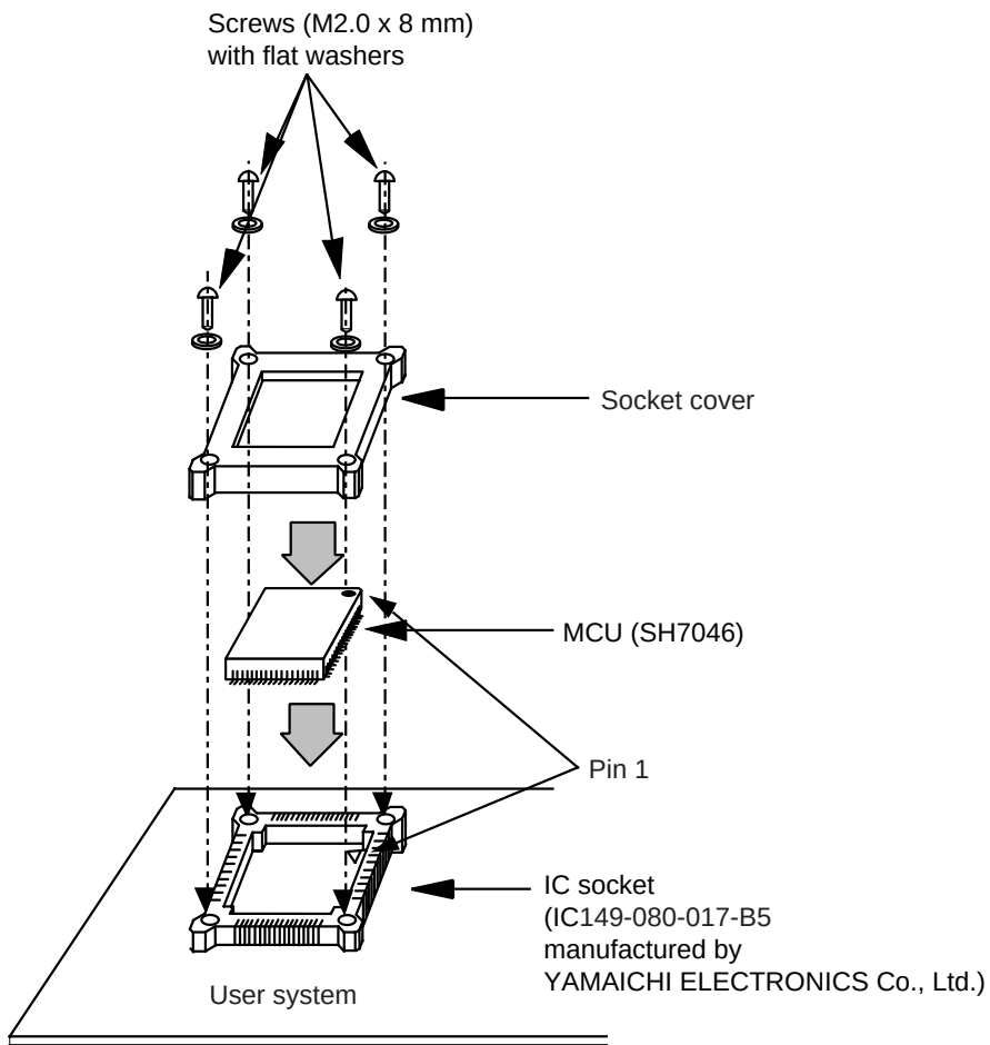
Figure 7 Installing MCU to User System
