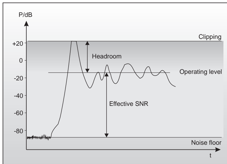
Fig. 3.2: The interactive relationship between the operating level and the headroom
