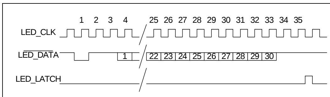
Figure 30. Mode 1 Timing
