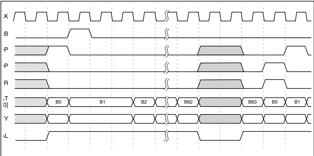
Figure 15. SPHY Receive Logical Timing
