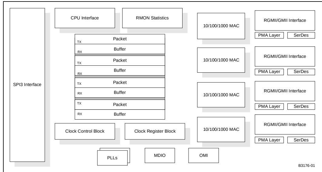
Figure 2. Internal Architecture
