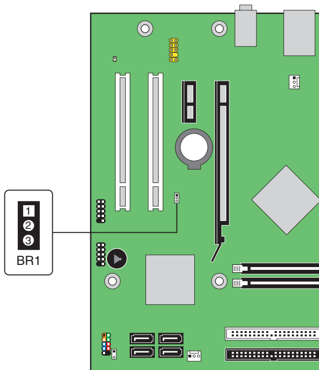
Figure 23. Location of the BIOS Configuration Jumper Block
