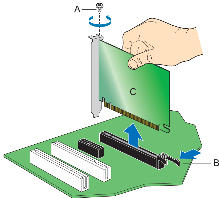
Figure 15. Removing a PCI Express x16 Card
