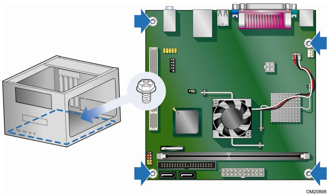
Figure 6. Desktop Board D945GCLF Mounting Screw Holes
