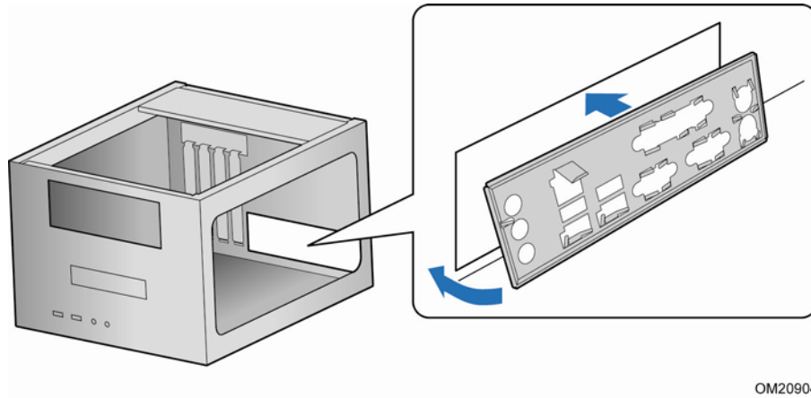
Figure 5. Installing the I/O Shield
