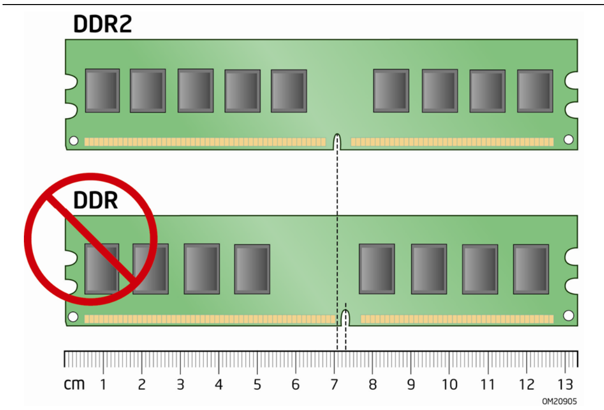
Figure 7. Use DDR2 DIMMs
