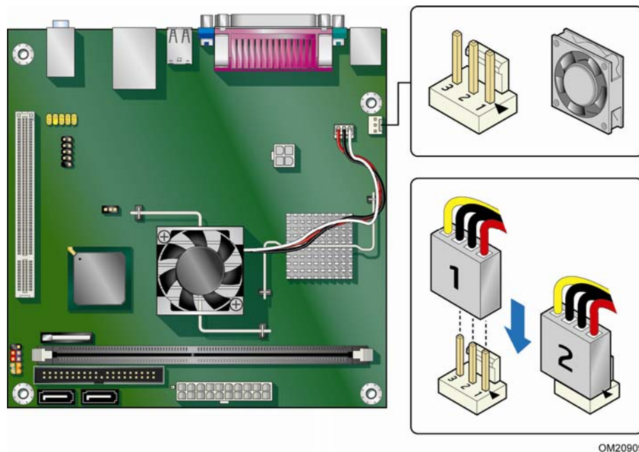
Figure 12. Location of the Chassis Fan Header
