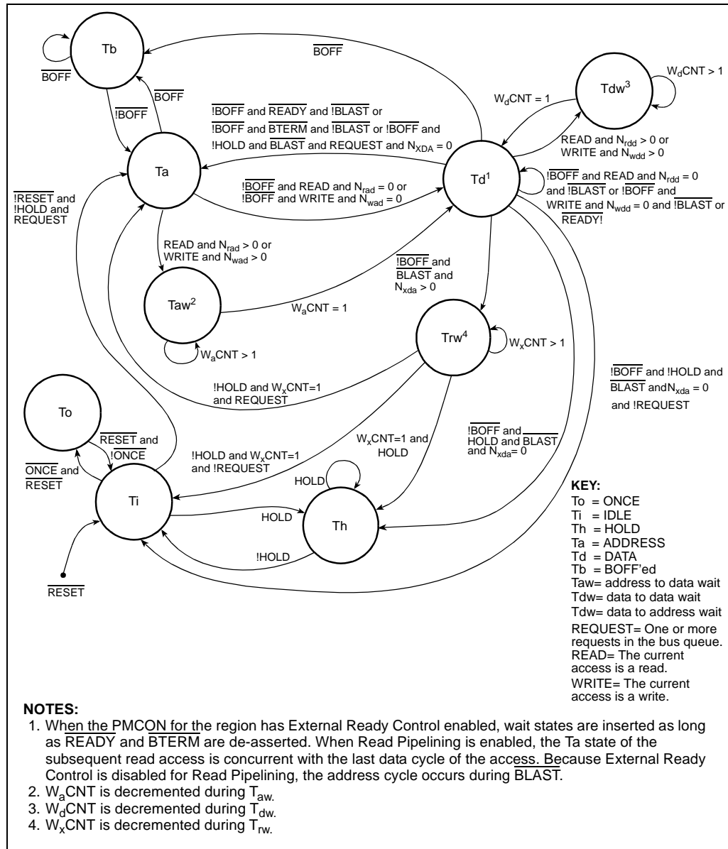
Figure 59. Bus States
