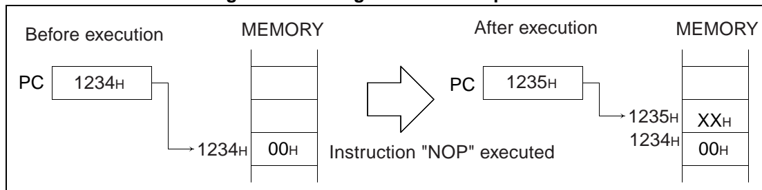
Figure 3.2-1 Program Counter Operation
