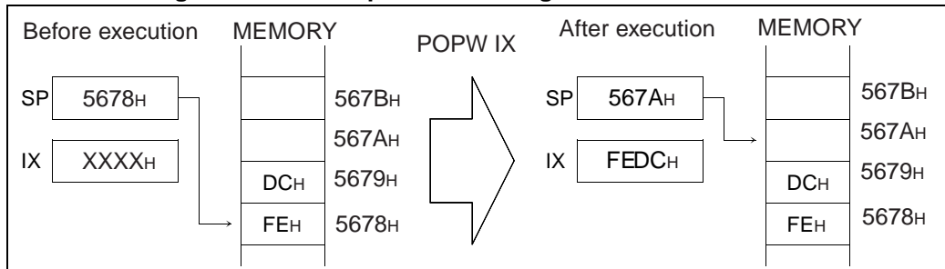
Figure 2.2-4 Example of Returning Data from Stack Area
