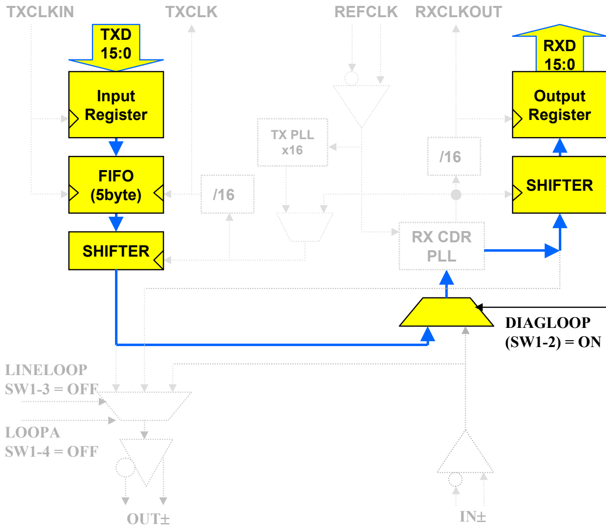
Figure 4. Diagnostic Loopback Mode Data Path
