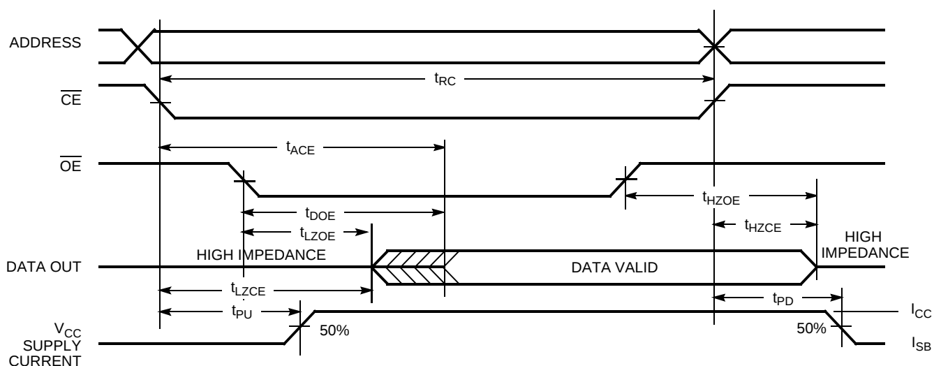
Figure 4. Read Cycle No. 2 ( \overline{OE} Controlled) [3, 14, 15]
