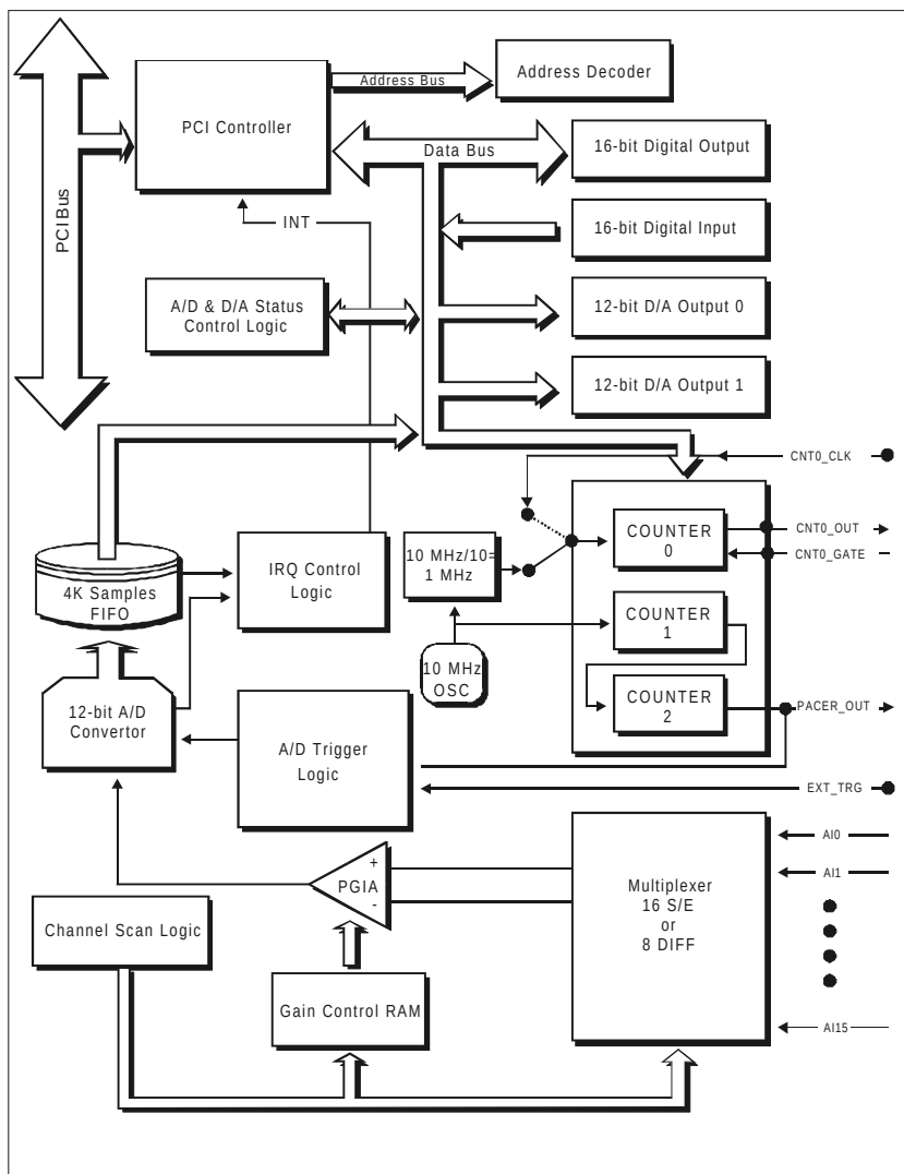
Figure 1-1: PCI-1710/PCI-1710HG block diagram
